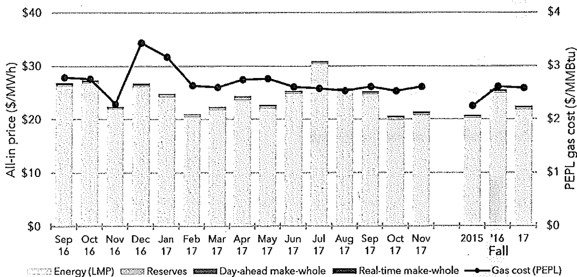
Figure 2-23 All-in cost
