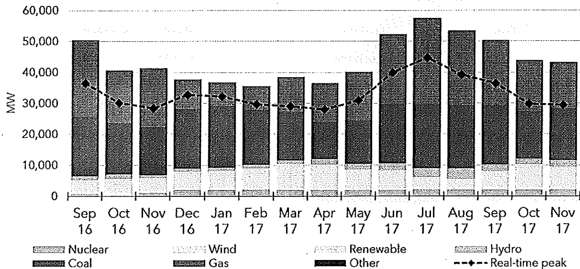
Figure 3–12 Hourly offered capacity, real-time average
