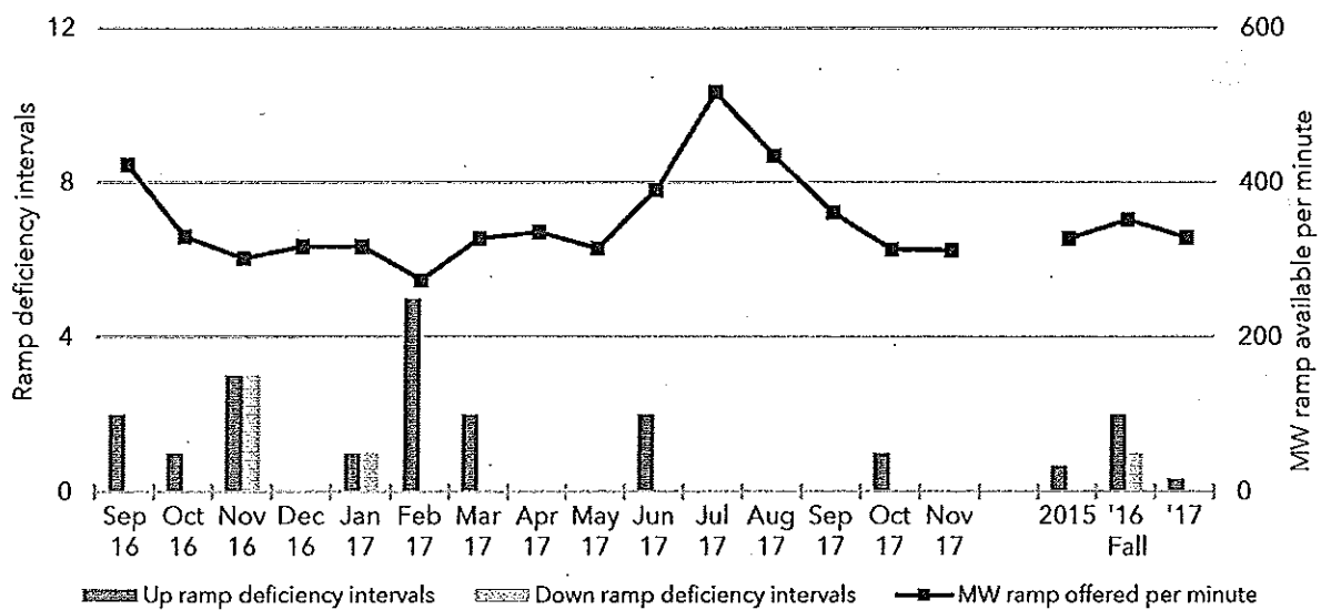
Figure 3–11 Ramp offered and deficiency intervals
