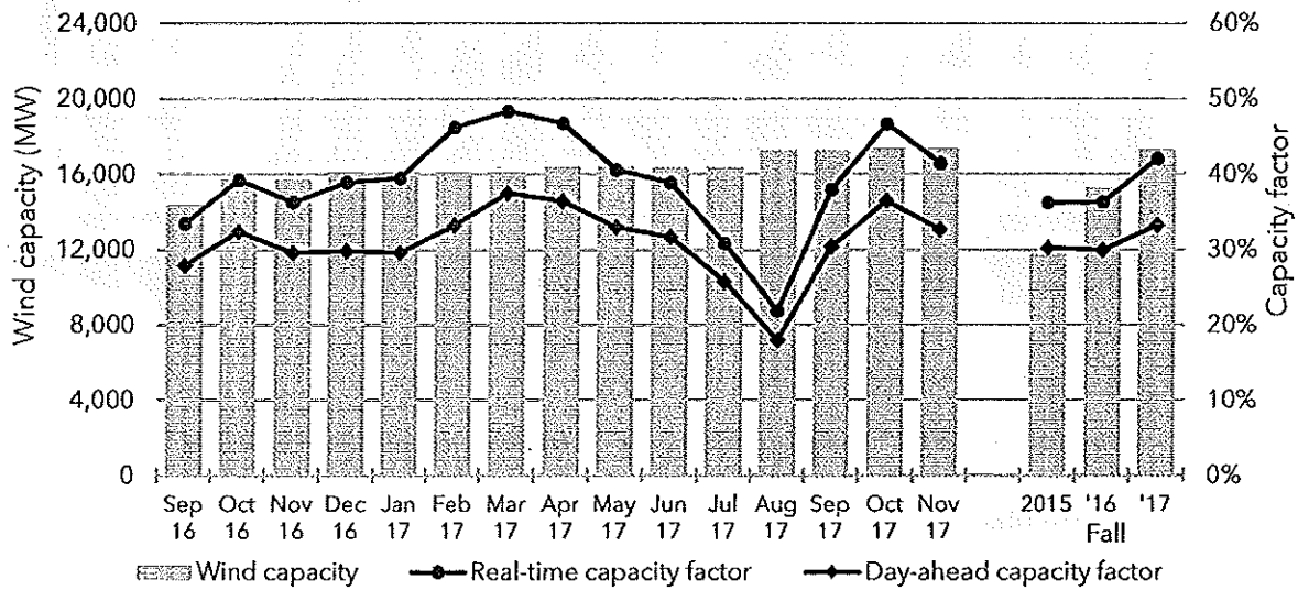
Figure 3–7 Wind capacity and capacity factor
