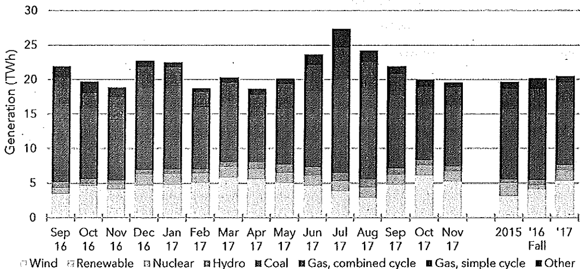
Figure 3-5 Generation by technology type, real-time
