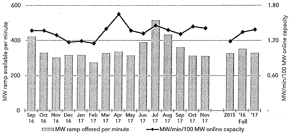
Figure 3–10 Ramp rate offered
