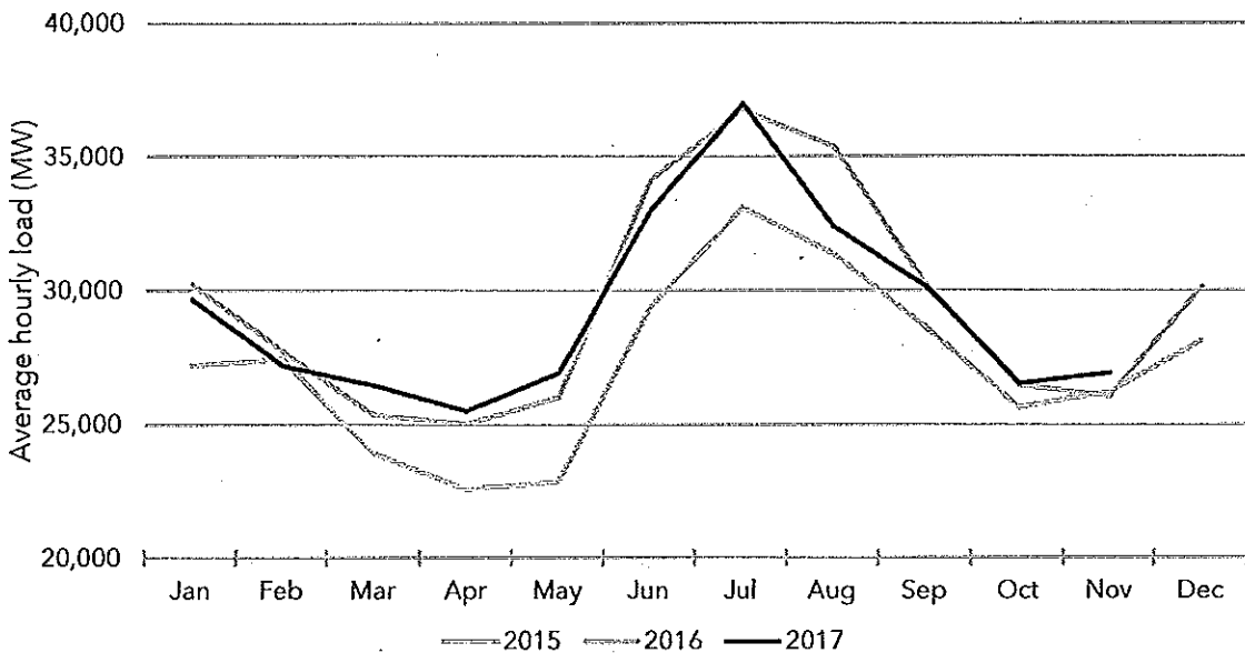
Figure 3–1 Average hourly load
