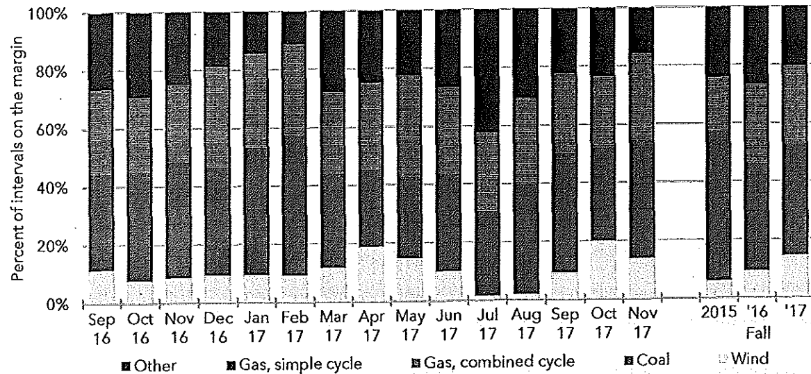
Figure 3–9 Technology on the margin, real-time
