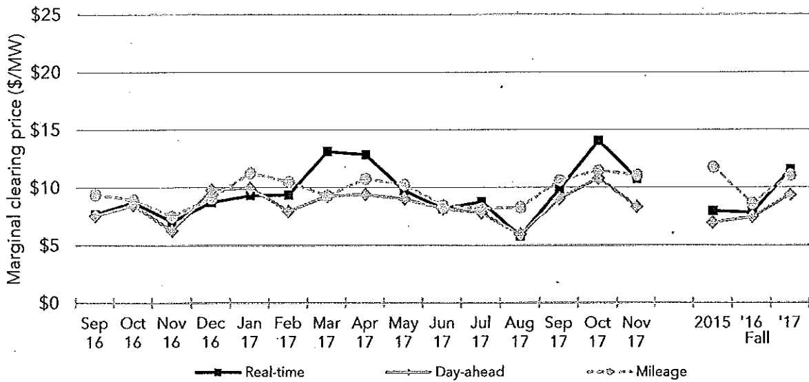
Figure 2–8 Regulation-up prices
