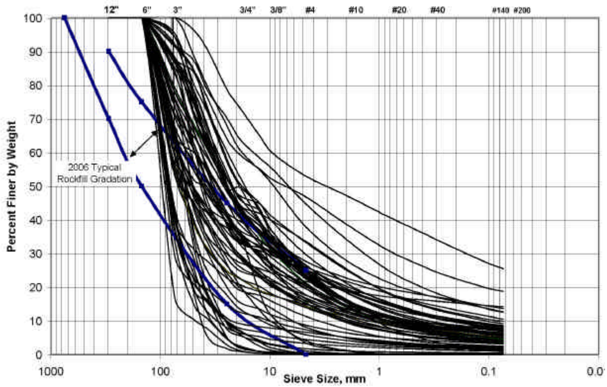
FIGURE 7-4 ROCKFILL GRADATION (6\"
