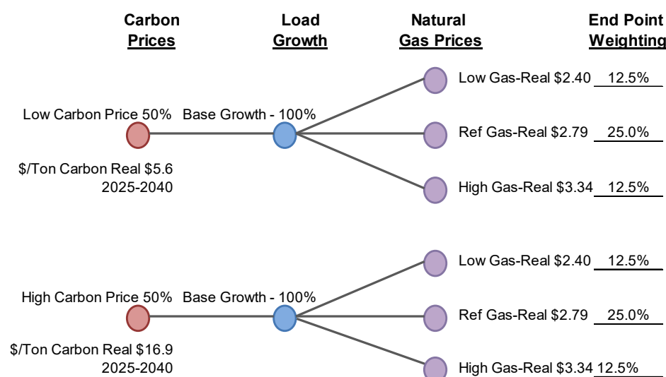
Figure 3.7: Scenario Tree
