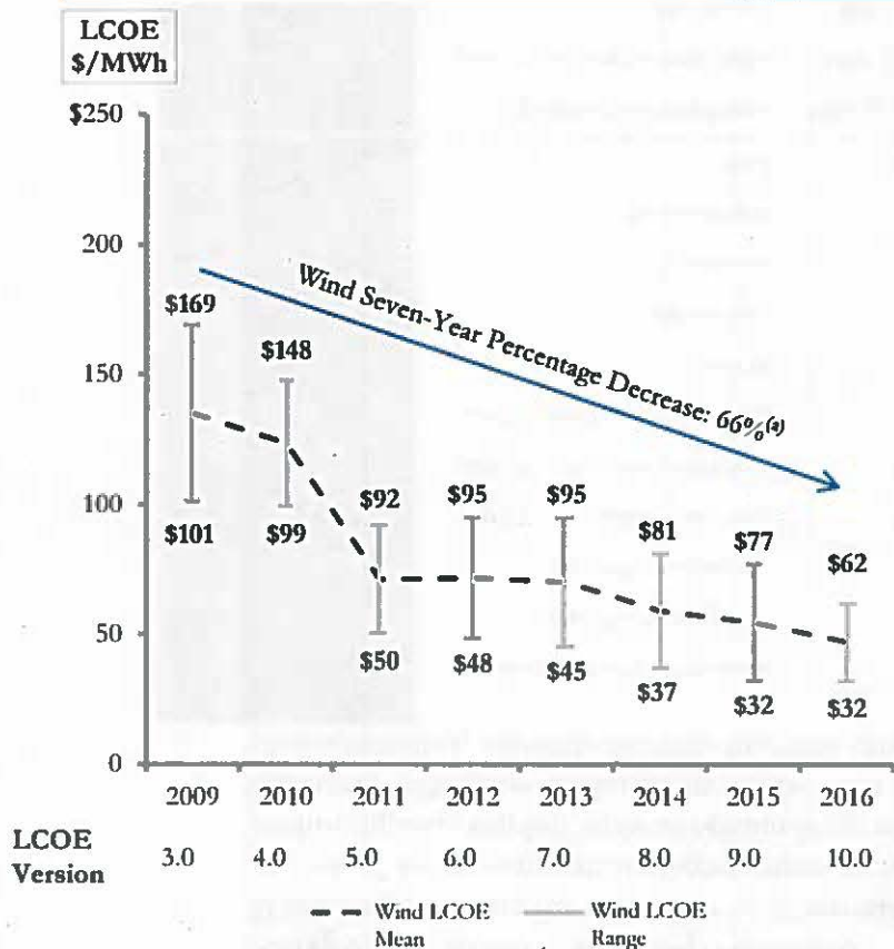
WIND LCOE
