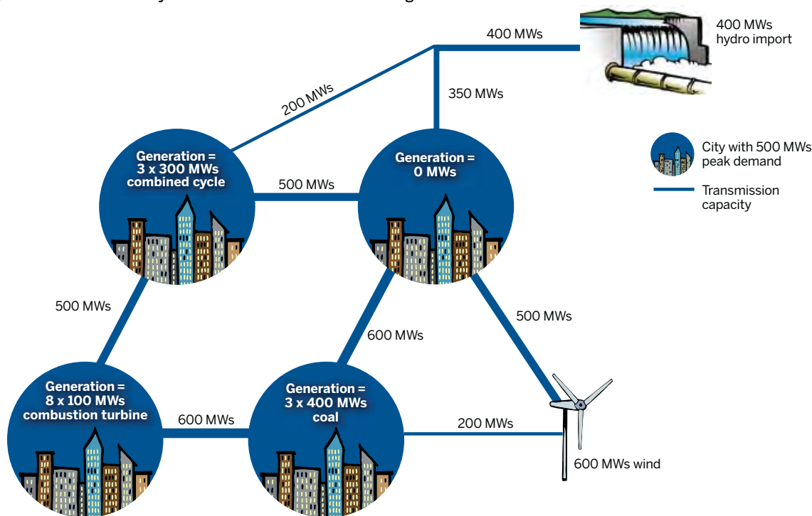
Figure 38. Transmission system with remote and centralized generation
