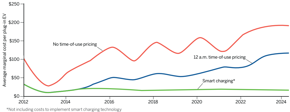
Figure 26. Estimated grid integration costs for electric vehicles
