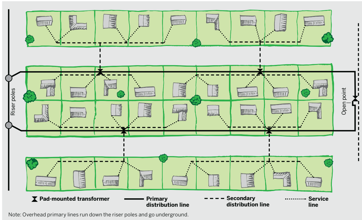
Figure 9. Underground distribution circuit with radial secondary lines
