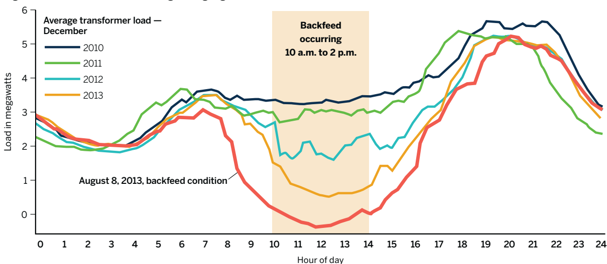
Figure 28. Substation backfeeding during high solar hours
