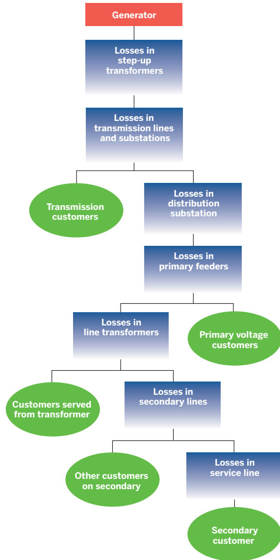
Figure 12. Electric delivery system line losses
