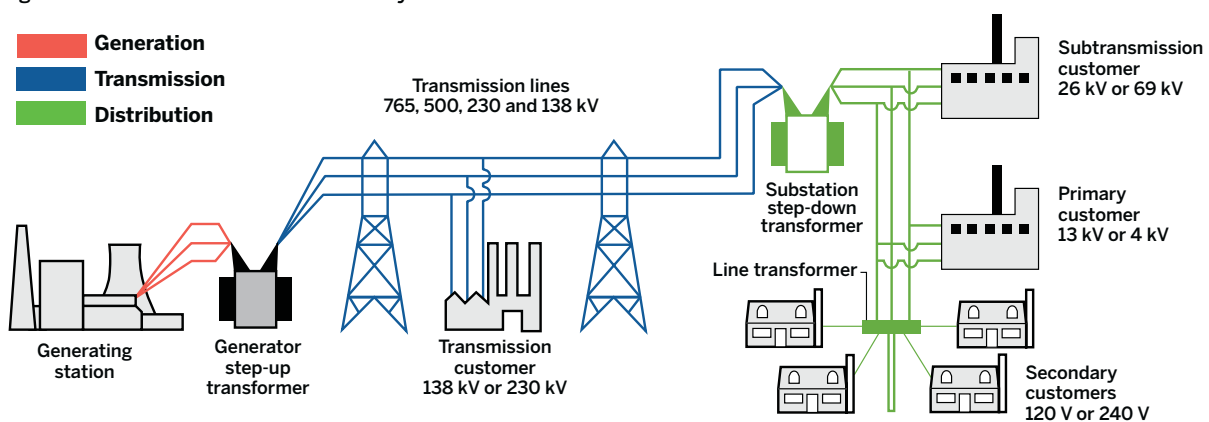
Figure 7. Illustrative traditional electric system
