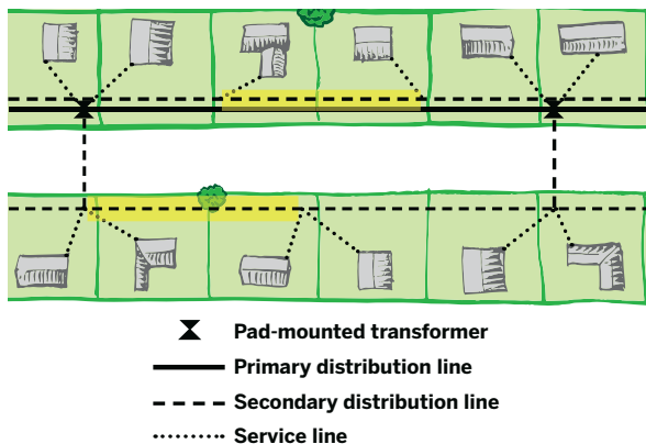
Figure 10. Detail of underground distribution circuit with networked secondary lines
