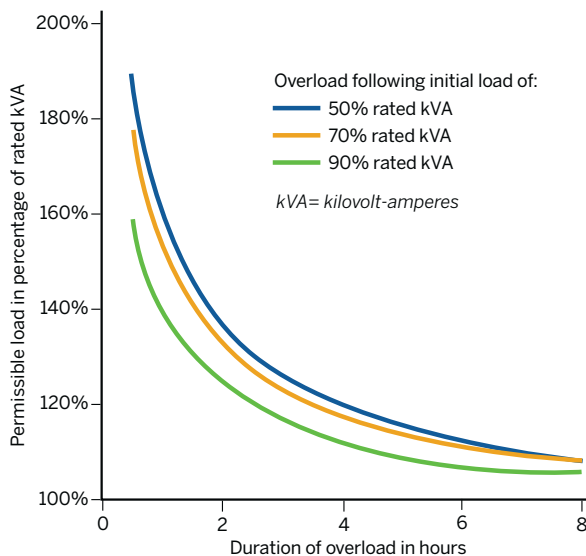
Figure 16. Permissible overload for varying periods
