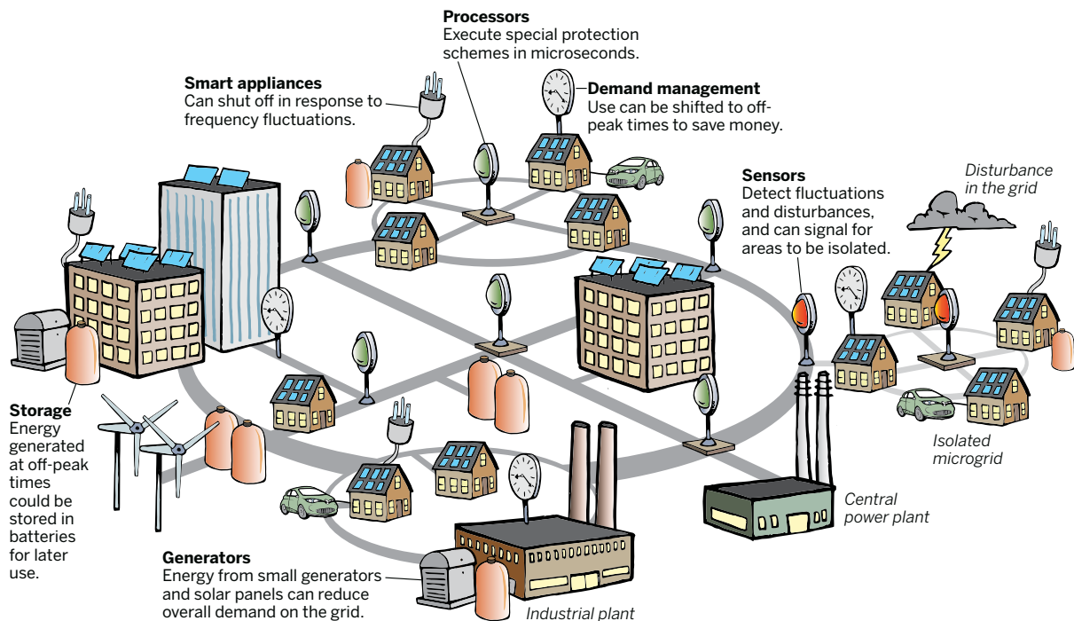
Figure 8. Illustrative modern electric system
