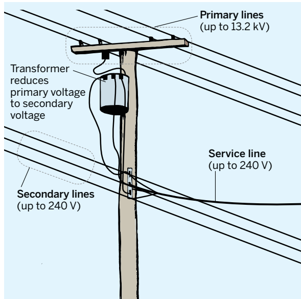
Figure 11. Secondary distribution pole layout
