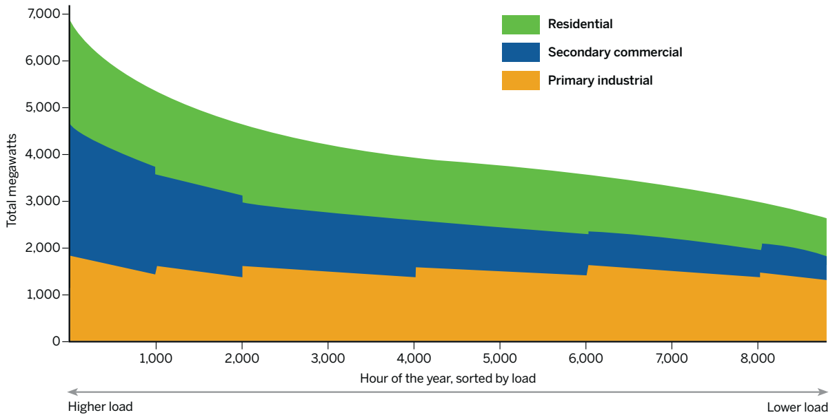
Figure 34. Illustrative customer class load in each hour
