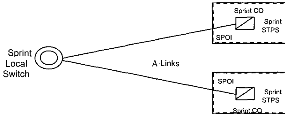
Figure 3. A-Link Interface
