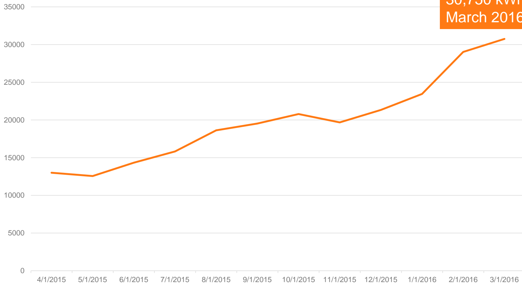
Energy (kWh) Monthly April 2015 - March 2016
