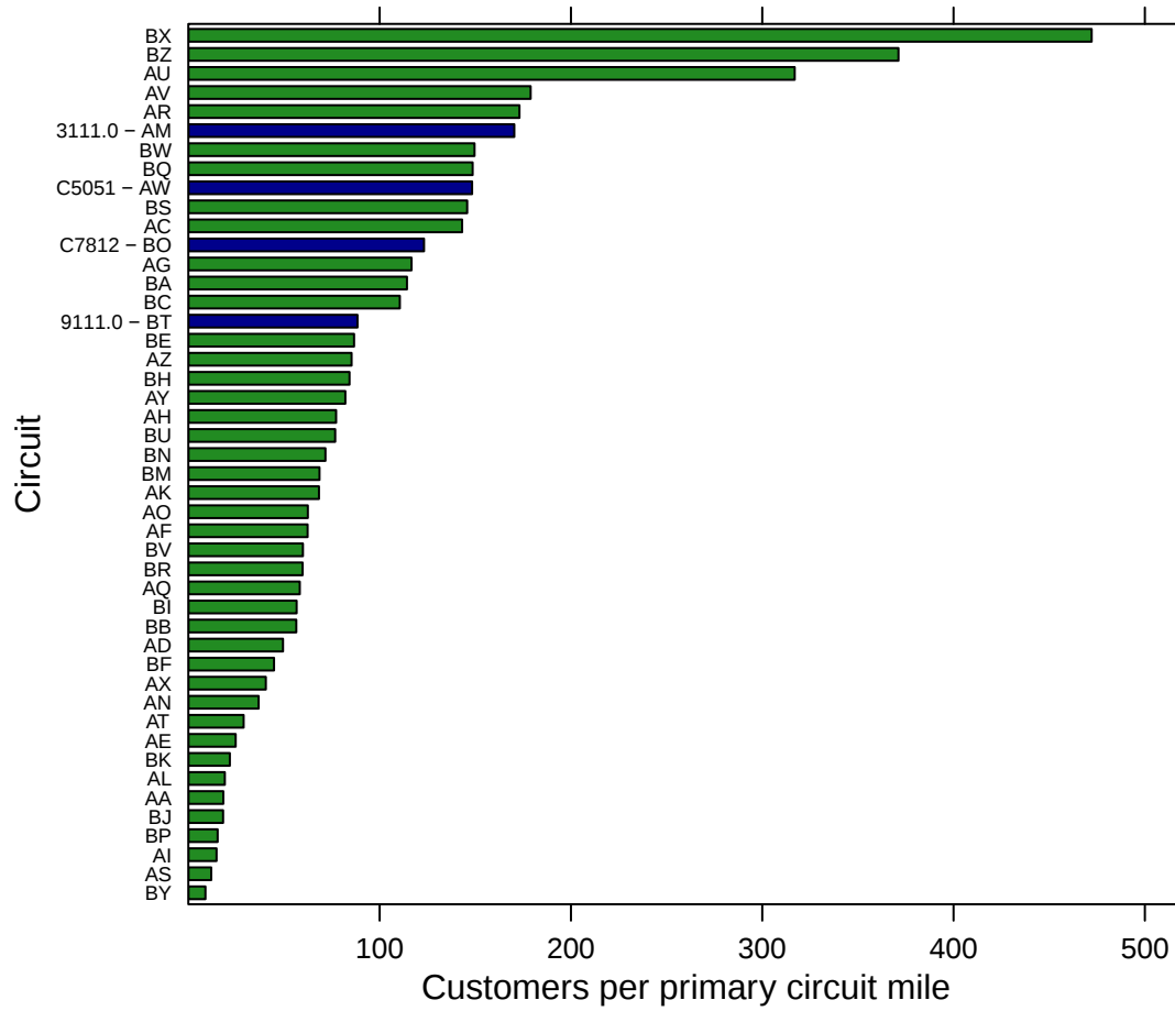
Figure 3-5 Load Densities
