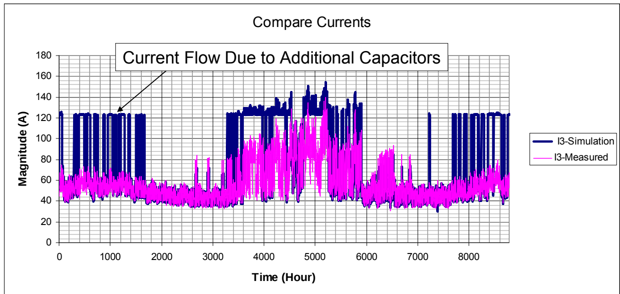
Figure 2-16 3111 Current Simulated vs. Measured (With Capacitor Controls)
