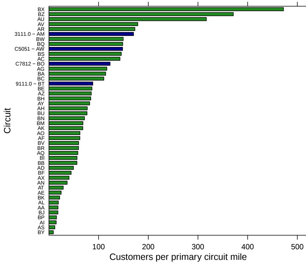
Figure 3-4 Load Densities
