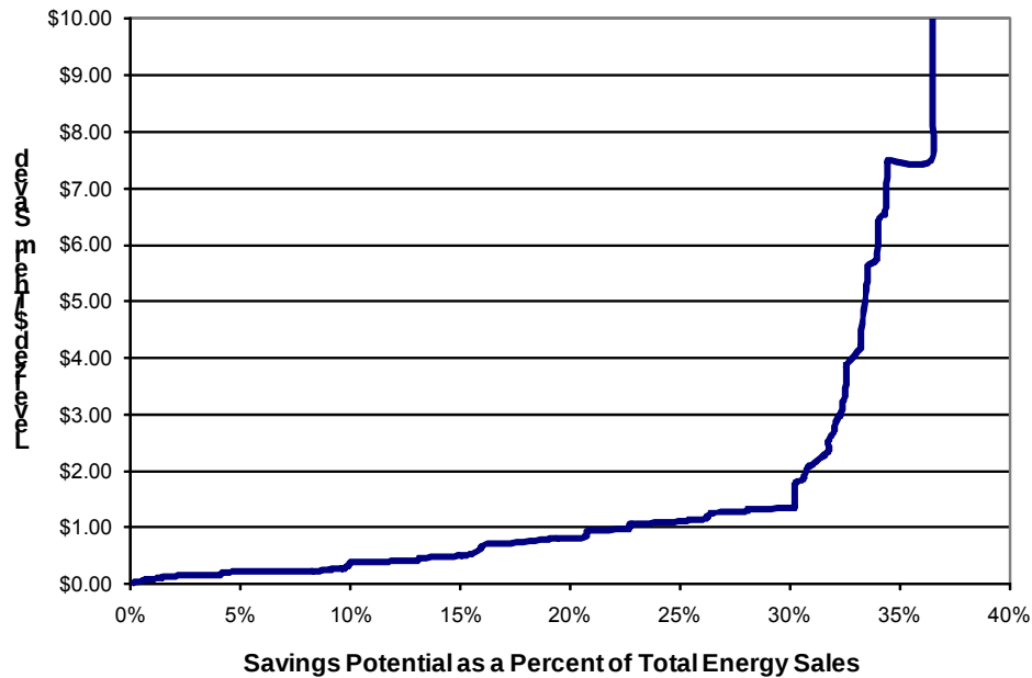
Figure 6-12 Natural-Gas Supply Curve*
