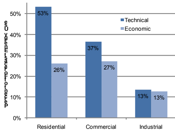
Figure 6-3 Technical and Economic Potential (2020) Percentage of 2020 Fixed-Efficiency Base Energy Use
