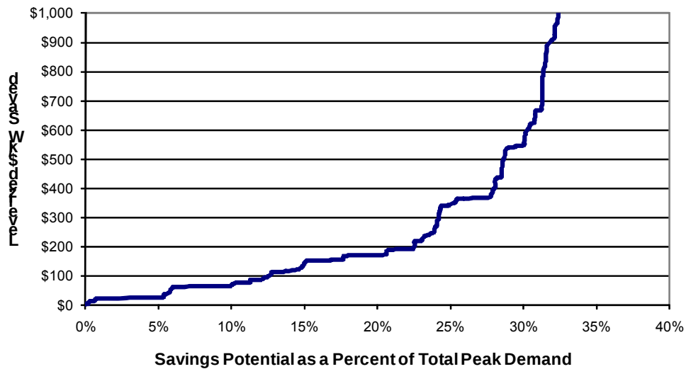
Figure 5-21 Peak-Demand Supply Curve*
