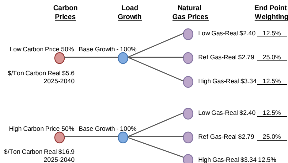
Figure 3.7: Scenario Tree
