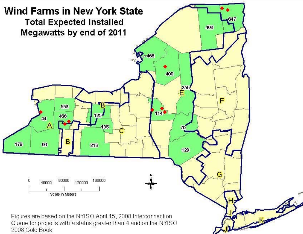
Figure 3-2: Distribution of Wind Interconnection Forecast
