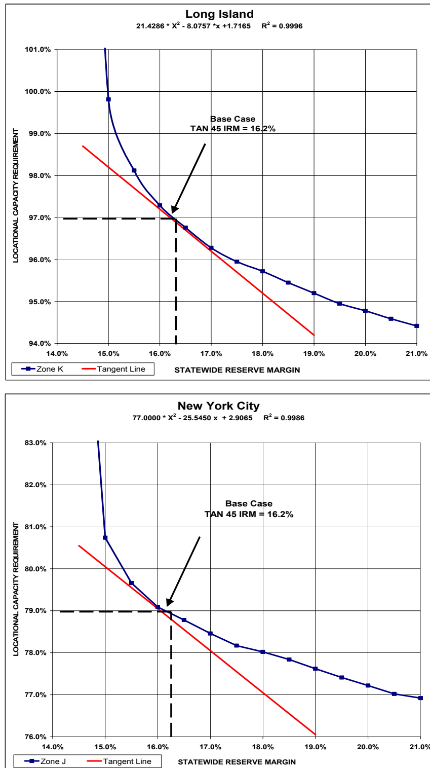
Figure 2: NYCA Locational ICAP Requirements vs. Statewide ICAP Requirements
