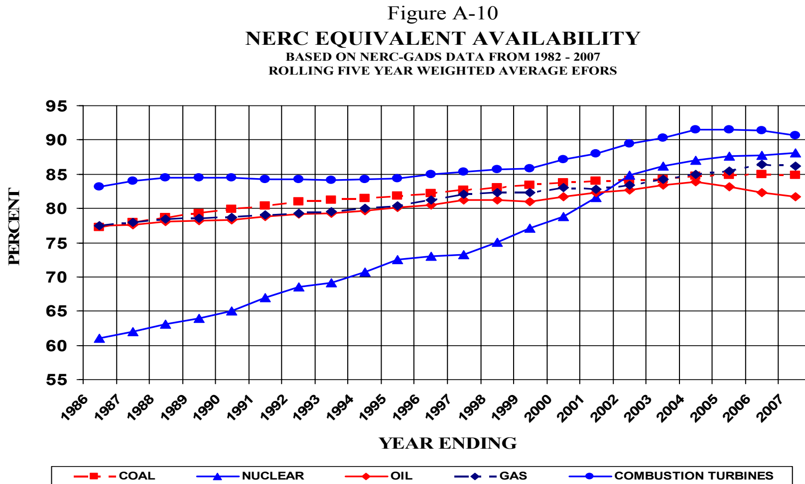
Figure A-10: NERC Region Equivalent Availability – 5 Year Rolling Average
