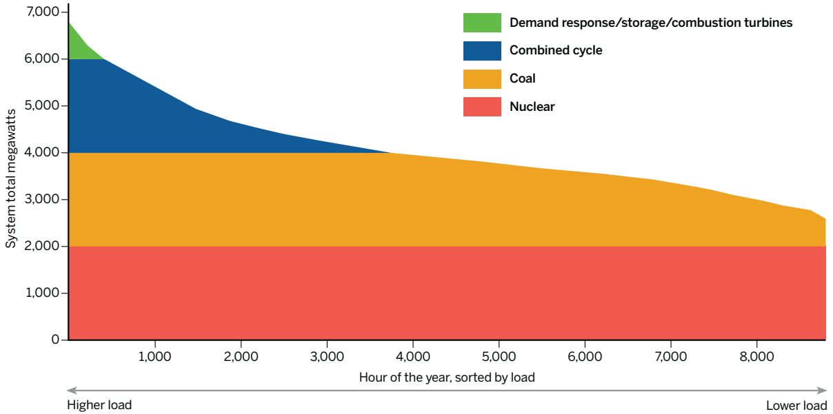
Figure 33. Simplified generation dispatch duration illustrative example
