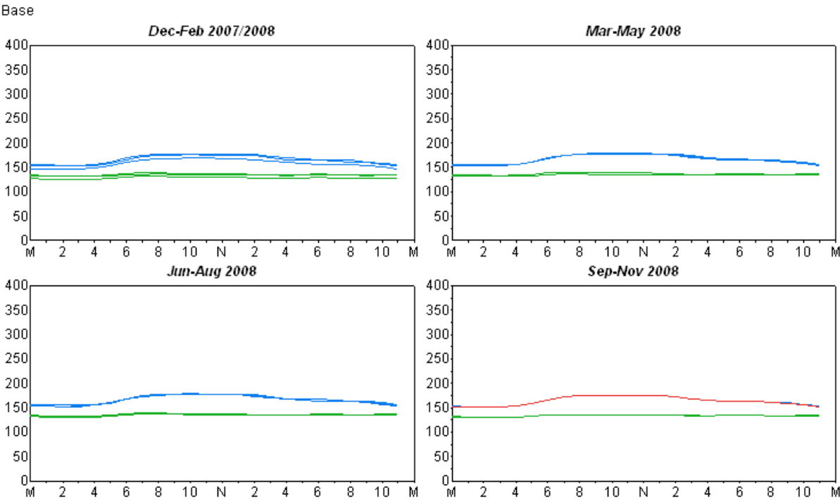
Figure 11: MPS Large Power Other Daytype Profile
