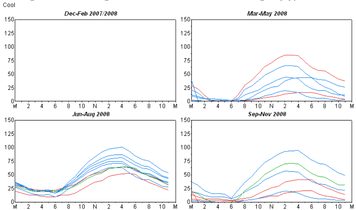
Figure 7: MPS Large General Service Air Conditioning Daytype Profile
