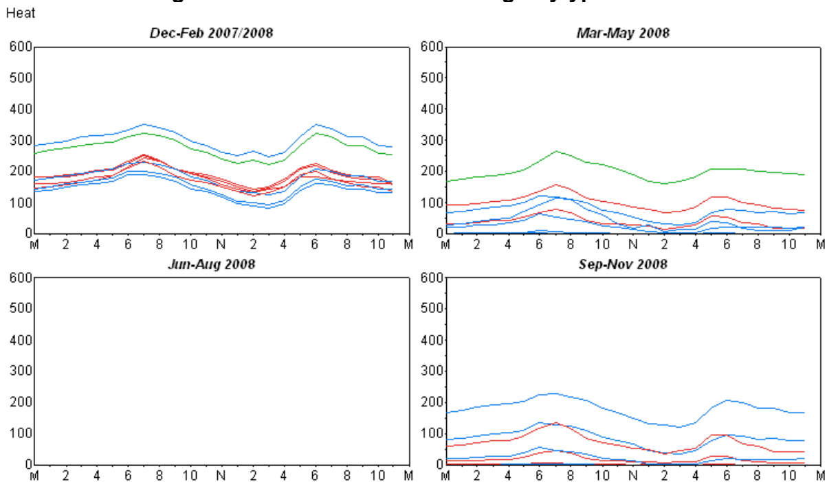
Figure 2: MPS Residential Heating Daytype Profile
