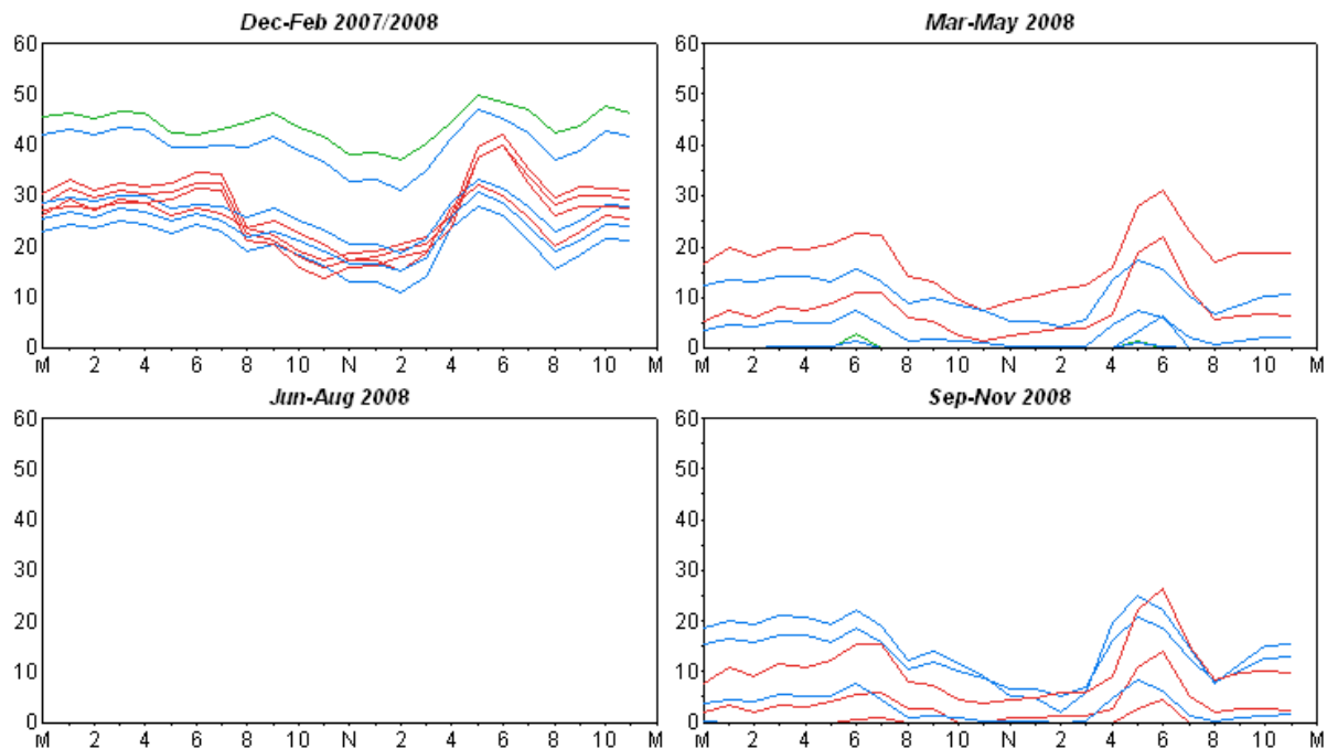
Figure 5: MPS Small General Service Heating Conditioning Daytype Profile
