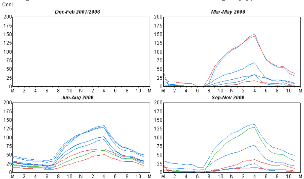
Figure 4: MPS Small General Service Air Conditioning Daytype Profile
