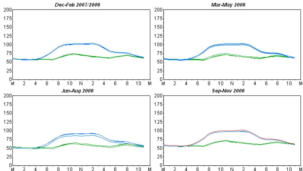
Figure 6: MPS Small General Service Other Daytype Profile
