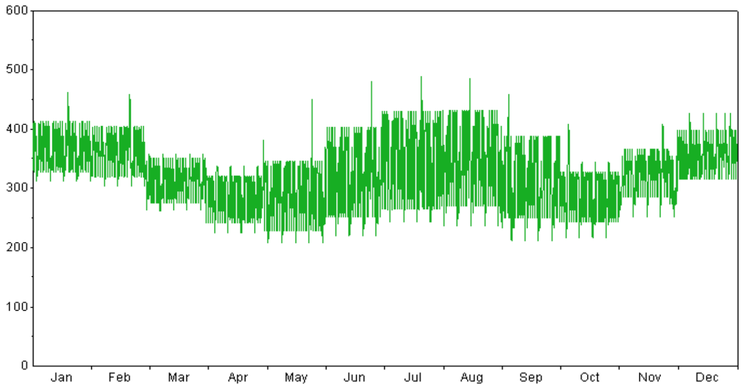
SJ Load Profile 2025
