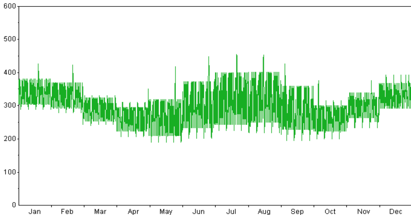
SJ Load Profile 2020
