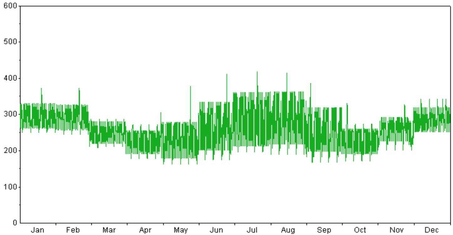
SJ Load Profile 2009
