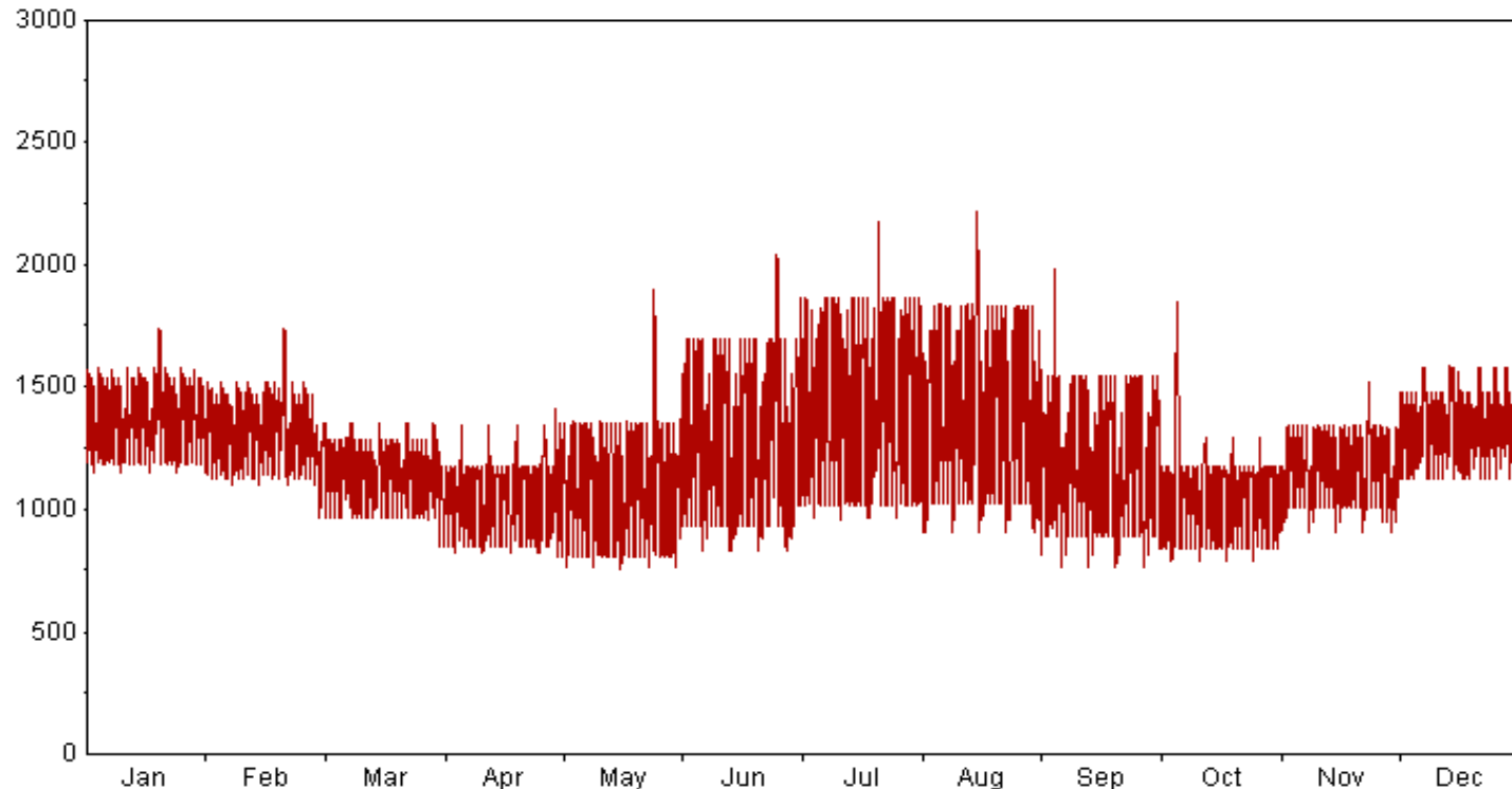
GMOC Load Profile 2023
