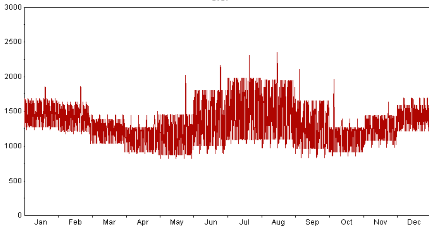
GMO Load Profile 2027
