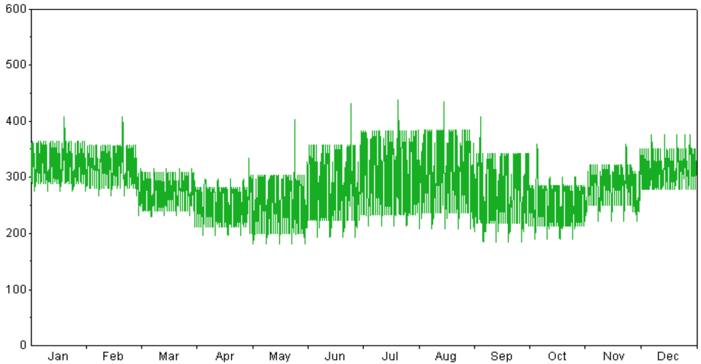
SJ Load Profile 2017
