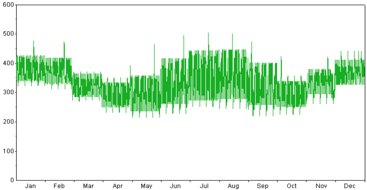
SJ Load Profile 2027
