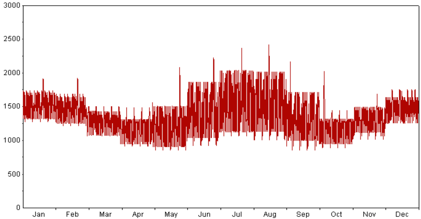
GMOC Load Profile 2029
