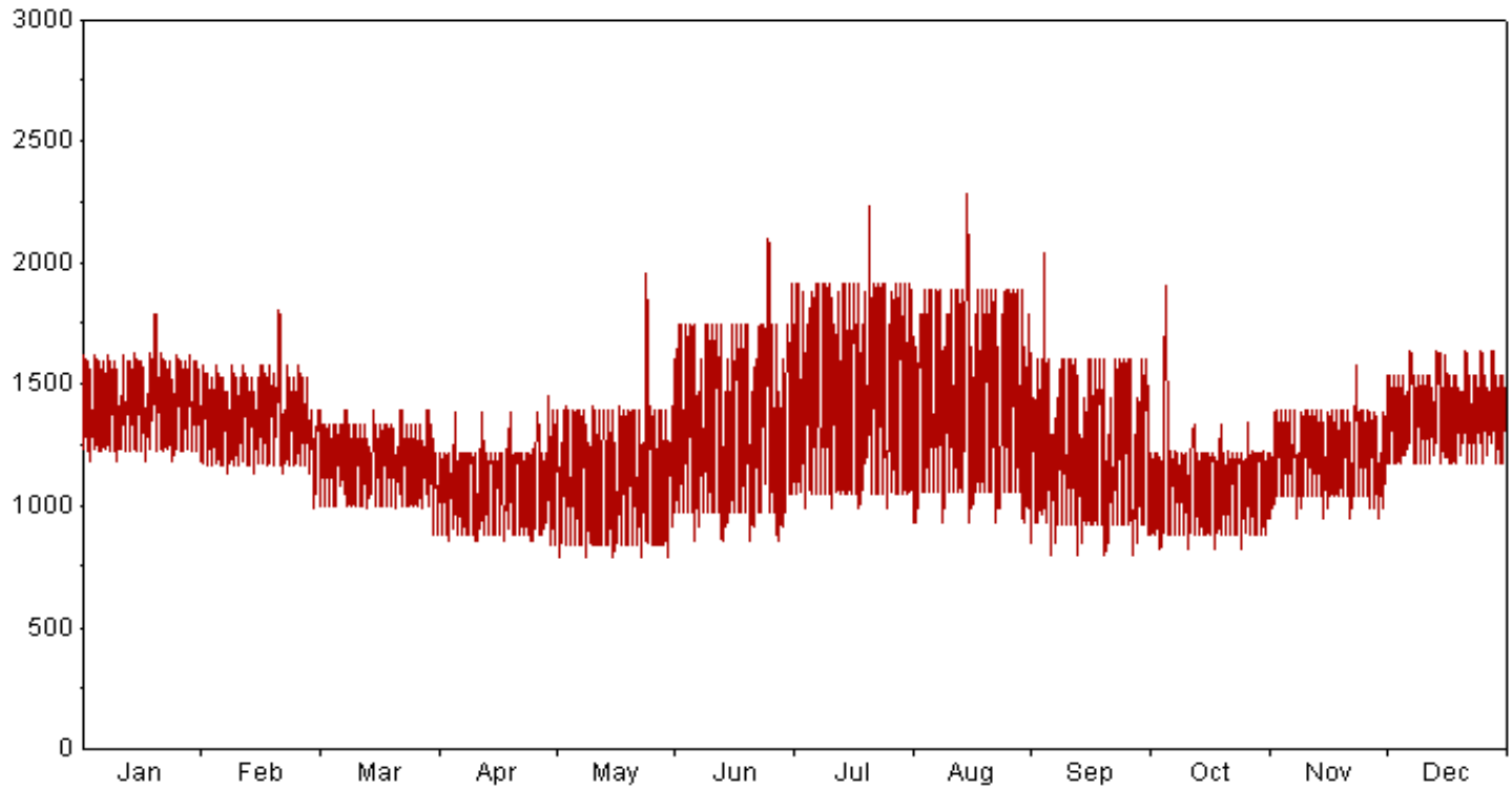
GMOC Load Profile 2025
