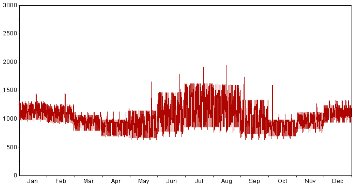
GMO Load Profile 2012
