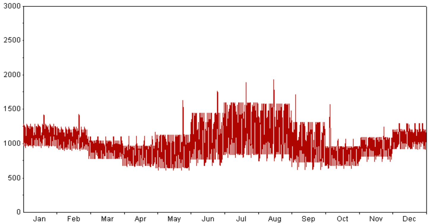
GMO Load Profile 2011
