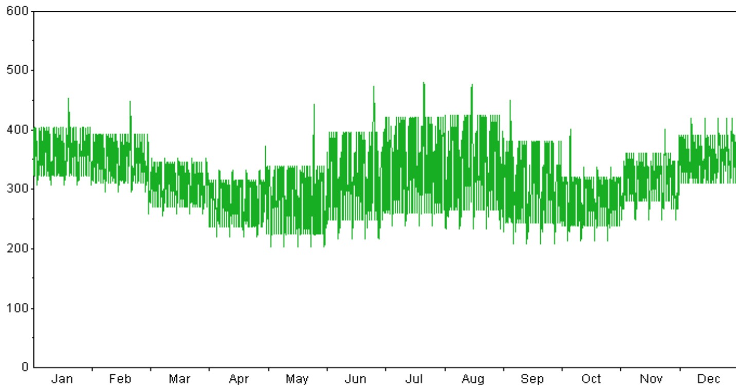
SJ Load Profile 2024
