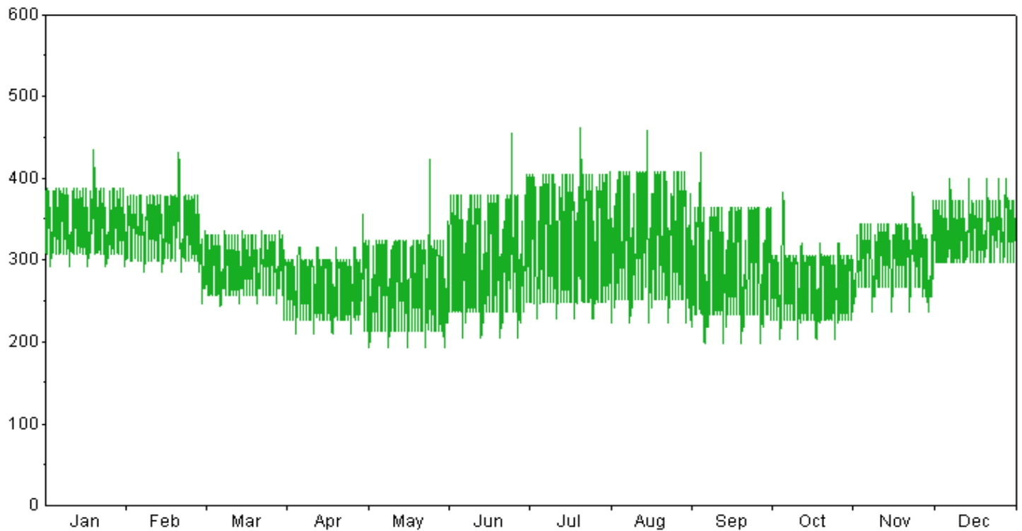
SJ Load Profile 2021
