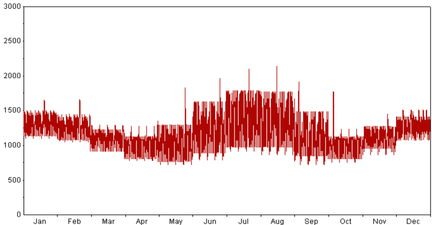
GMOC Load Profile 2020
