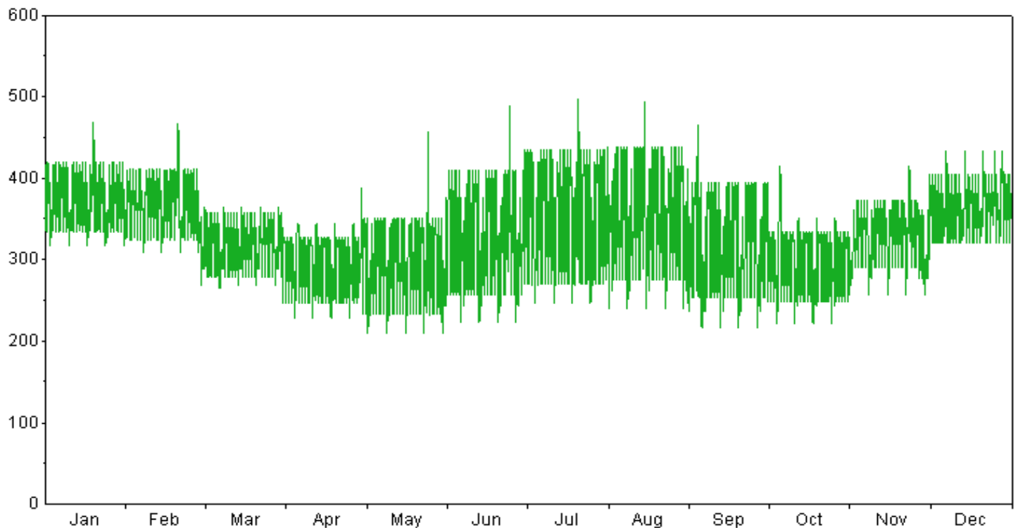
SJ Load Profile 2026
