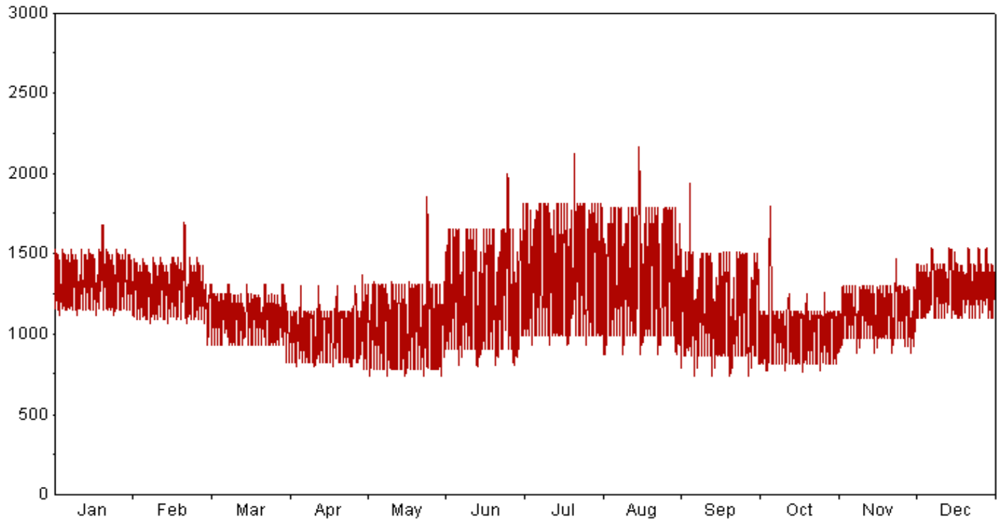
GMOC Load Profile 2021
