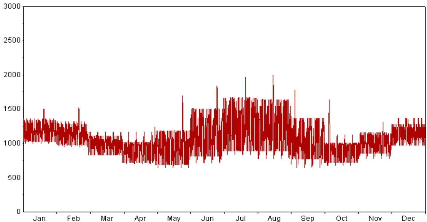
GMOC Load Profile 2014
