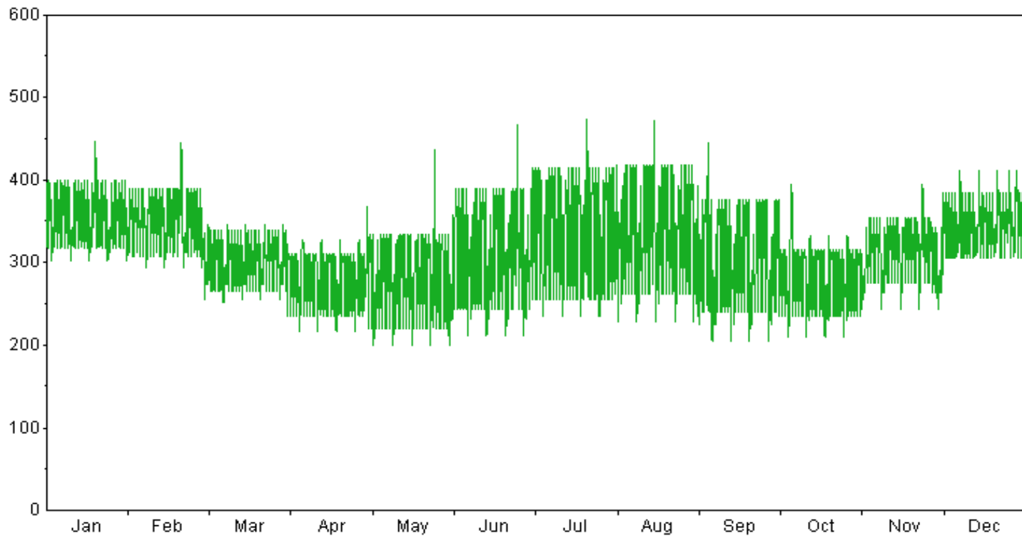
SJ Load Profile 2023
