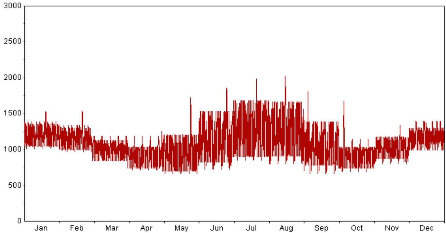
GMOC Load Profile 2015
