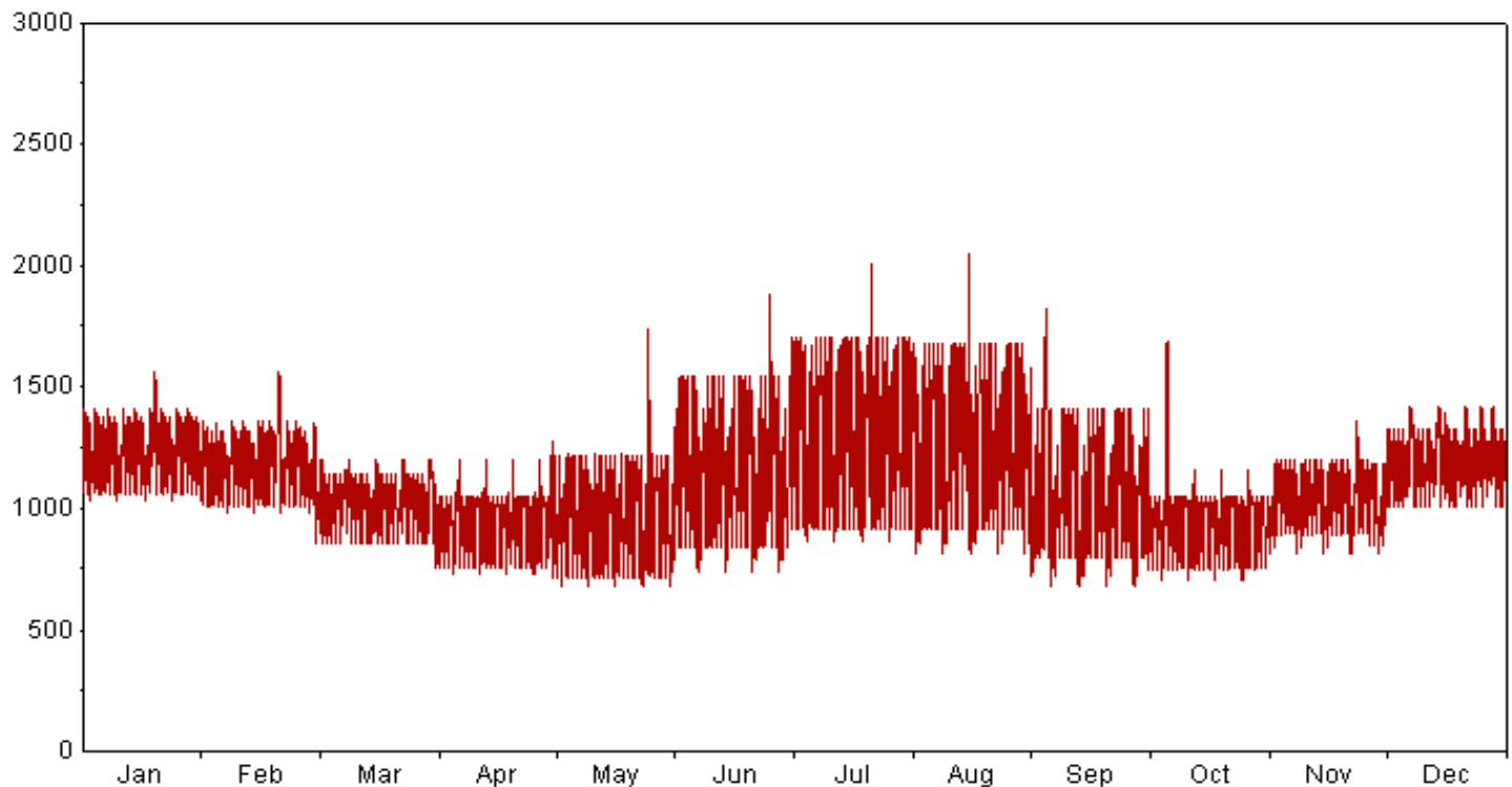
GMOC Load Profile 2016
