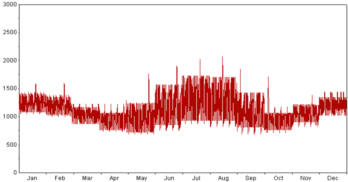
GMOC Load Profile 2017
