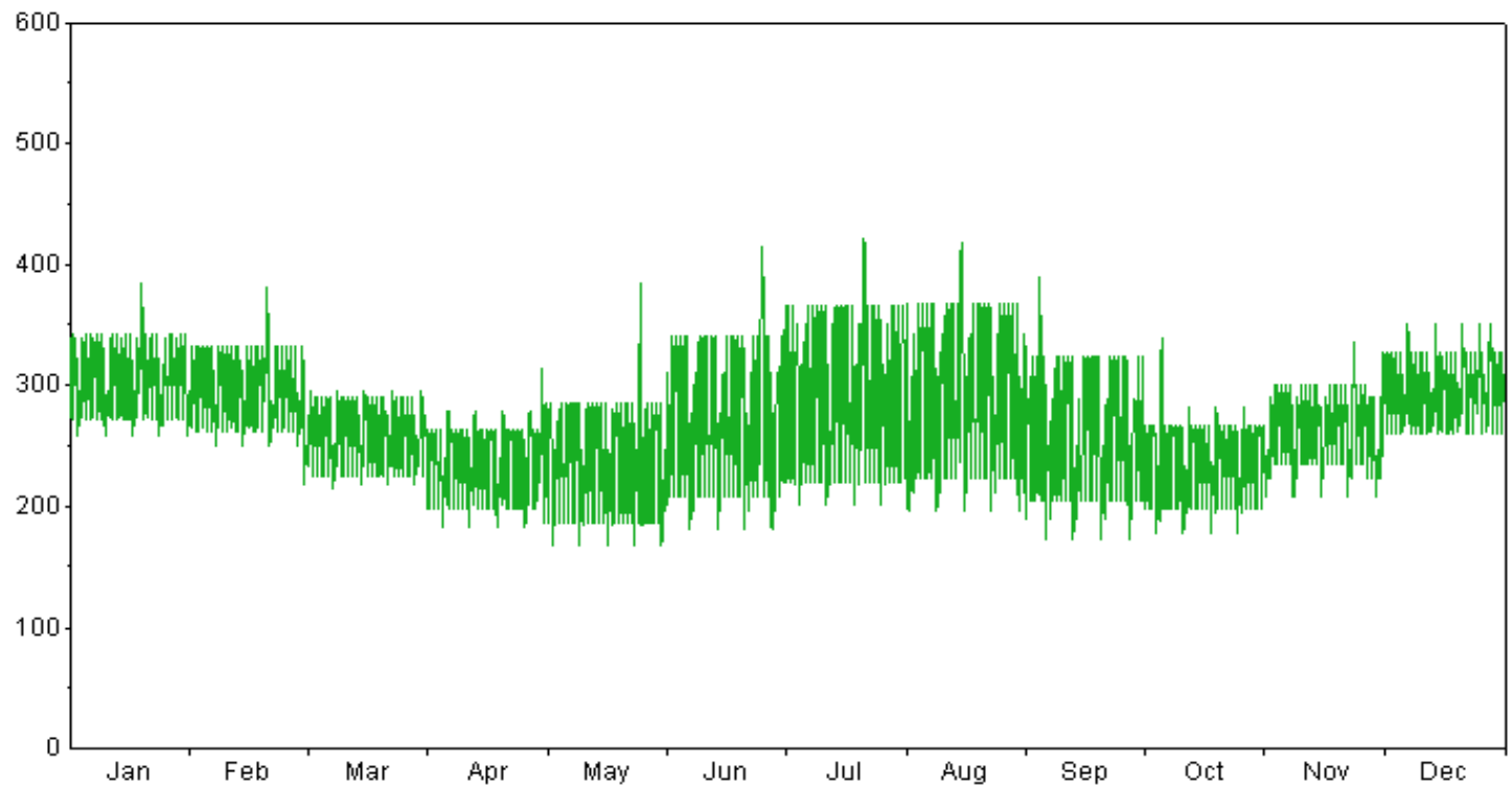
SJ Load Profile 2012
