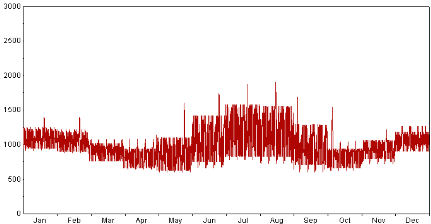
GMO Load Profile 2010
