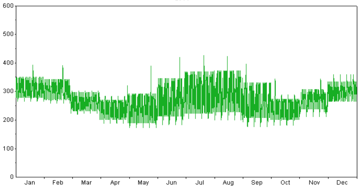
SJ Load Profile 2014
