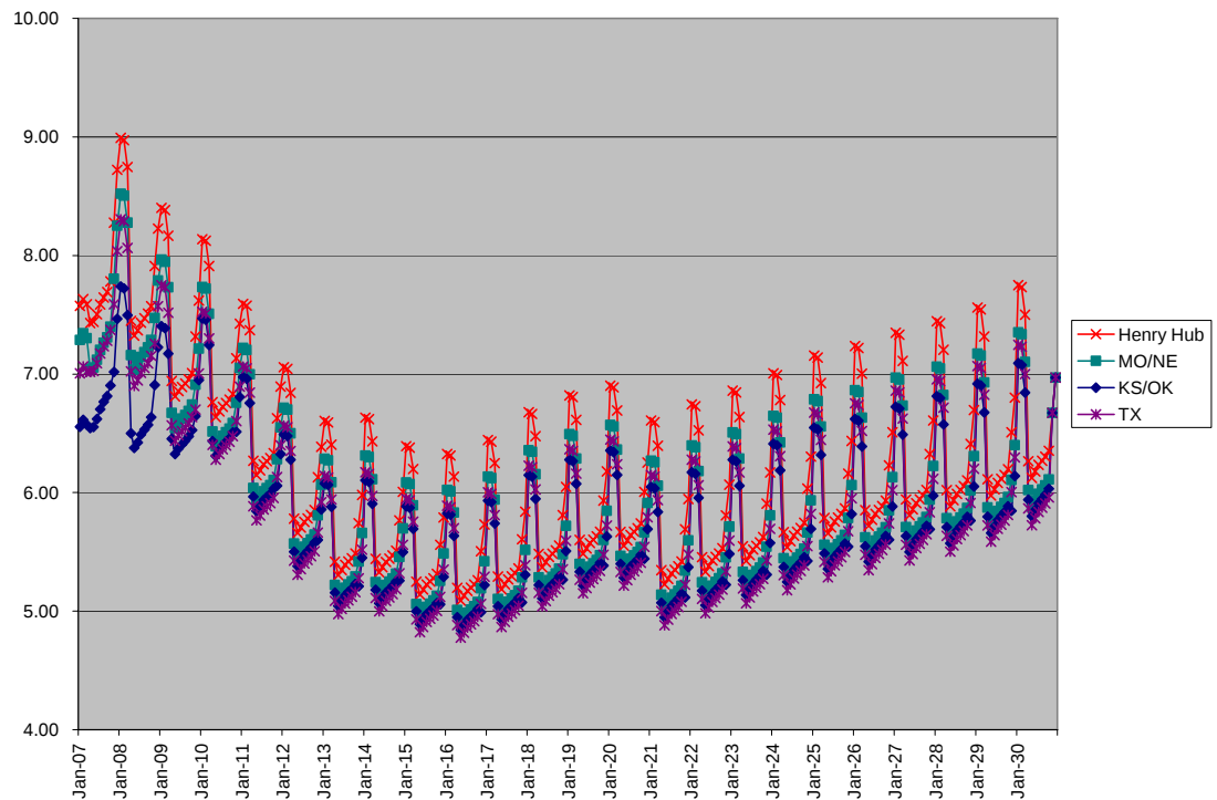
Figure 3. Forecast Regional Natural Gas Prices (Real 2005 $/MMBtu)
