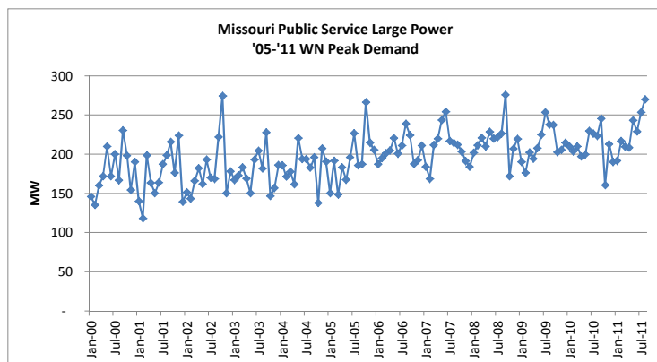
Plot 3A1-4 Missouri Public Service Class Weather Normalized Peak Demand (MW)
