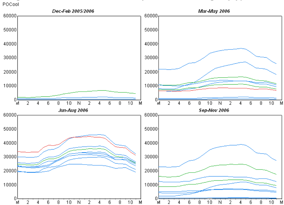
Figure 7: MO Commercial Primary Air Conditioning Daytype Profile
