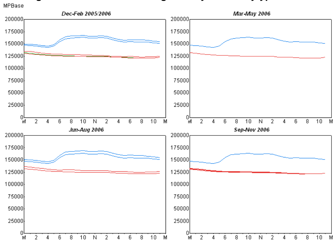
Figure 11: MO Manufacturing Primary Other Daytype Profile
