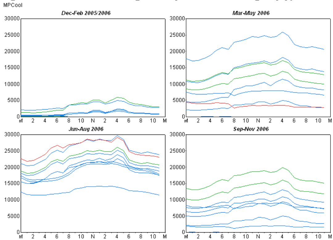
Figure 10: MO Manufacturing Primary Air Conditioning Daytype Profile
