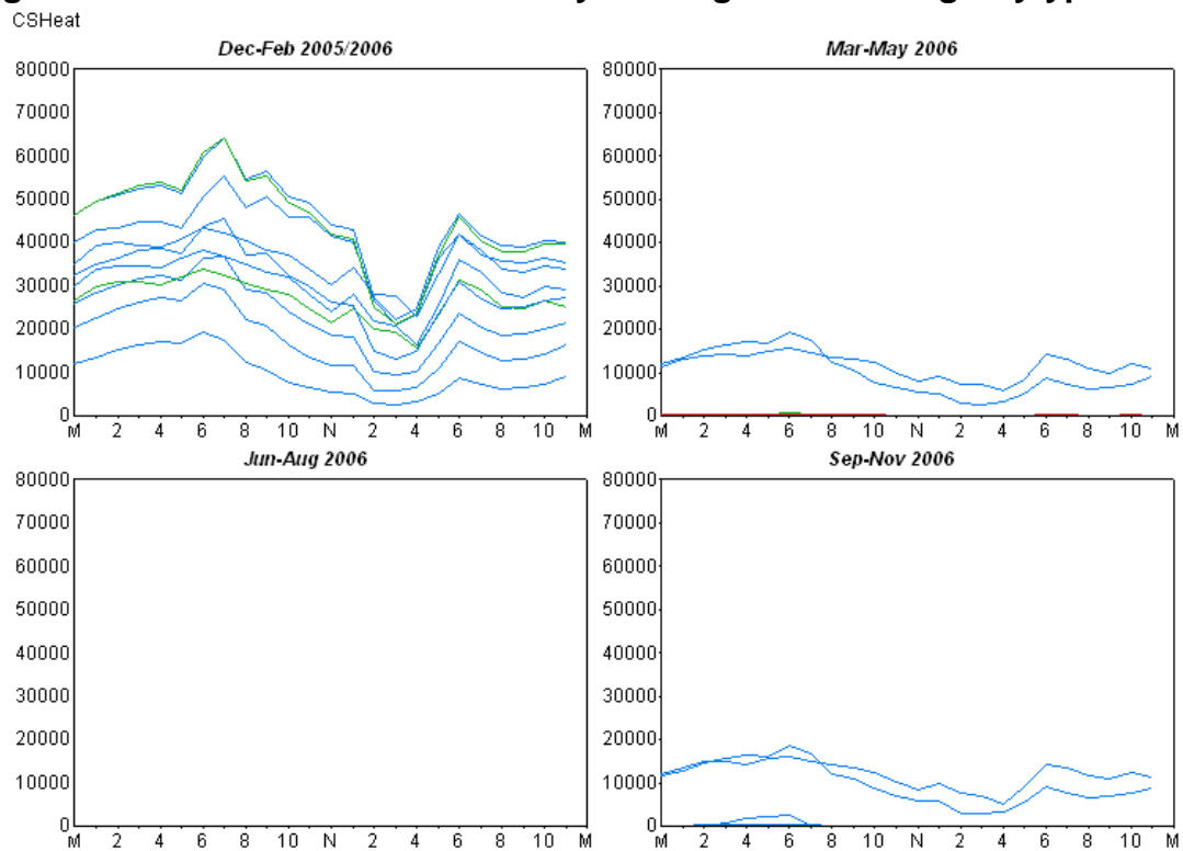
Figure 5: MO Commercial Secondary Heating Conditioning Daytype Profile
