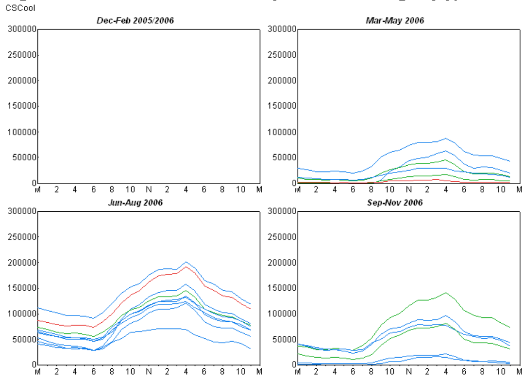
Figure 4: MO Commercial Secondary Air Conditioning Daytype Profile
