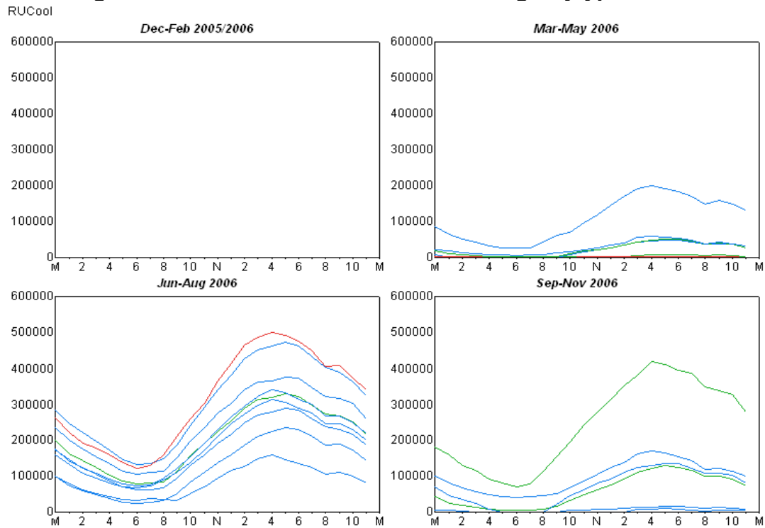
Figure 1: MO Residential Air Conditioning Daytype Profile
