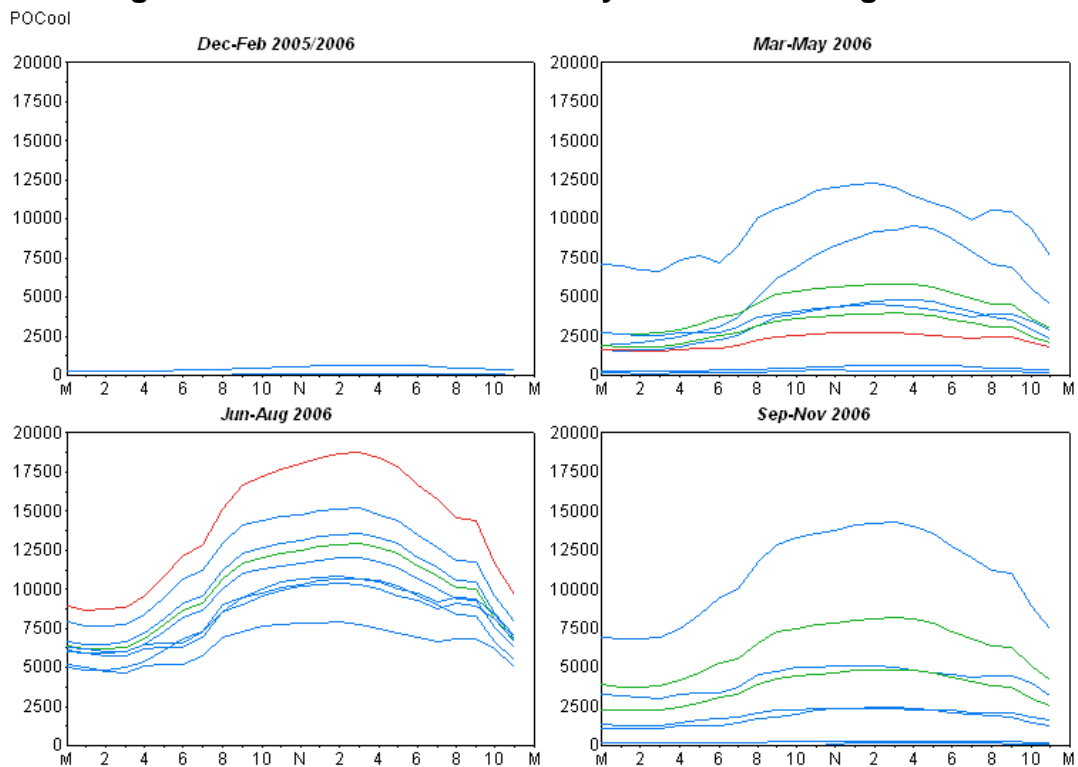
Figure 7: KS Commercial Primary Air Conditioning Profile
