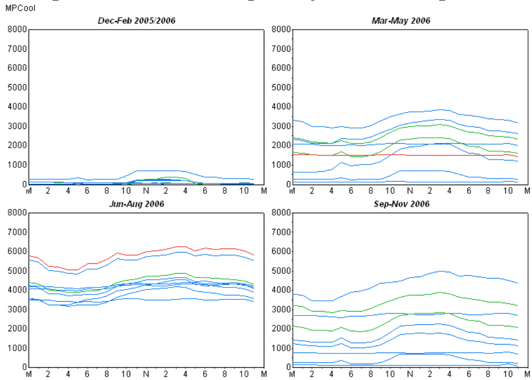
Figure 10: KS Manufacturing Primary Air Conditioning Profile
