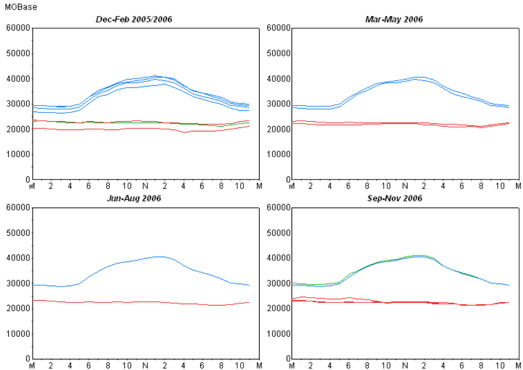
Figure 13: KS Manufacturing Other - Other Profile
