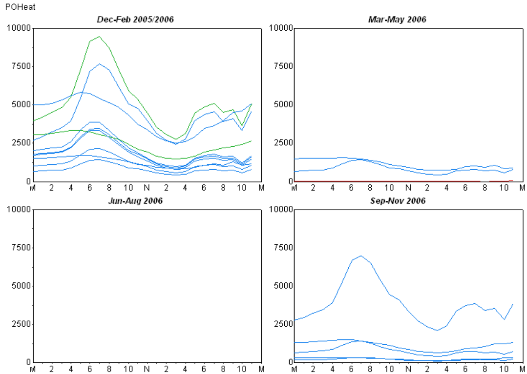
Figure 9: KS Commercial Primary Other Profile
