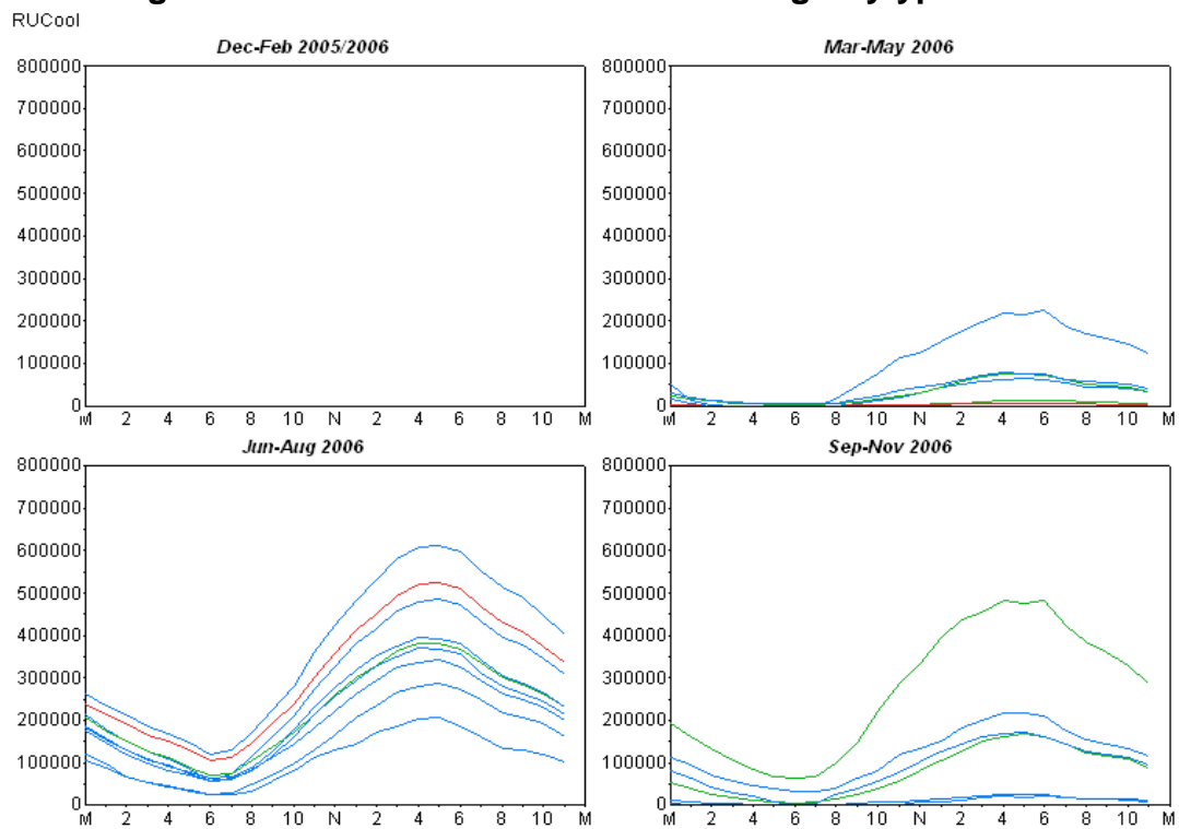
Figure 1: KS Residential Air Conditioning Daytype Profile
