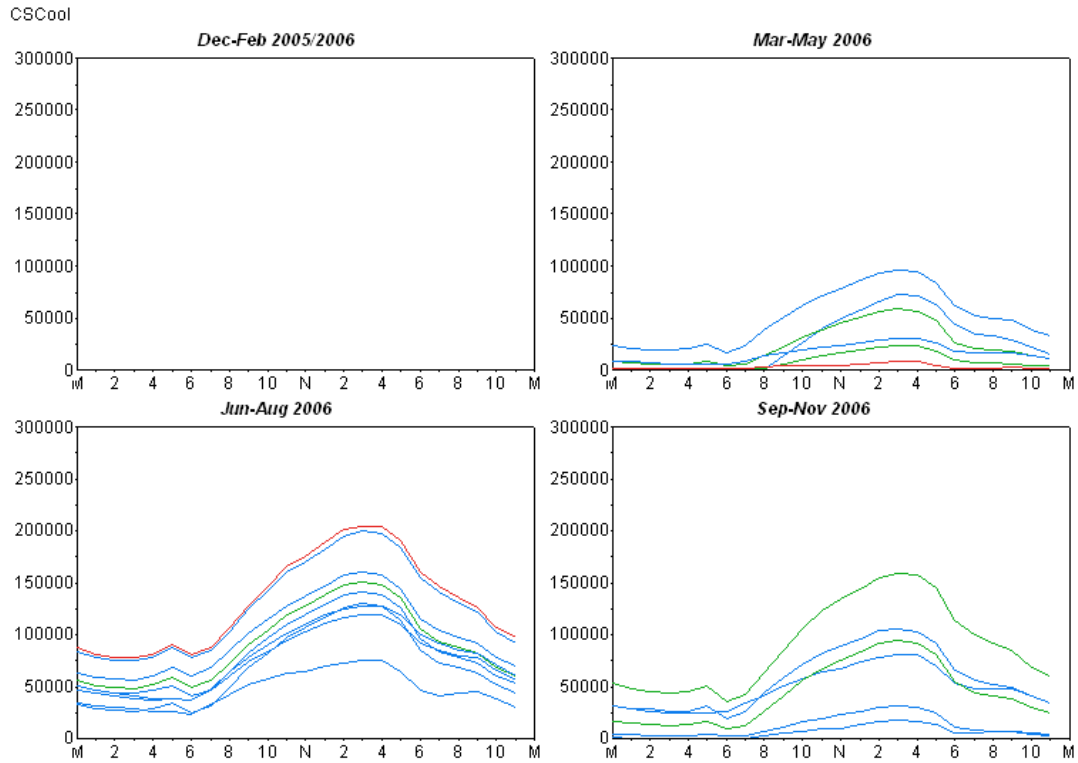
Figure 4: KS Commercial Secondary Air Conditioning Profile
