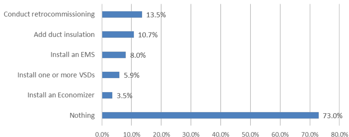
Figure 3-16 HVAC-Related Energy Efficiency Improvements Made in the Last 3 Years (N=752, All Respondents)
