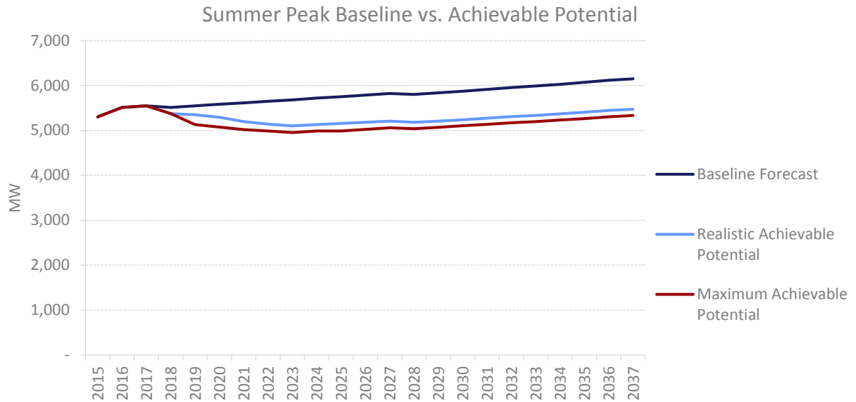
Figure 2-1 Baseline and Achievable DR & DSR Potential Forecasts (Summer Peak MW)
