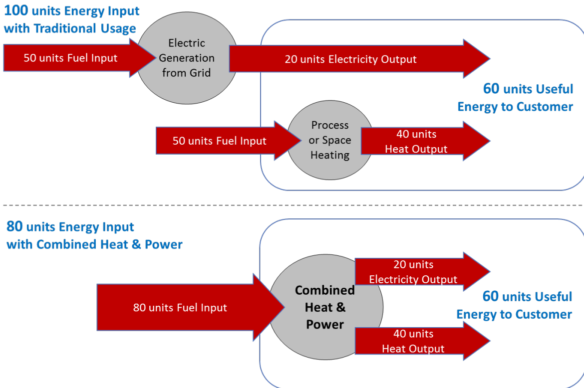
Figure 3-1 Review of CHP Energy Flows
