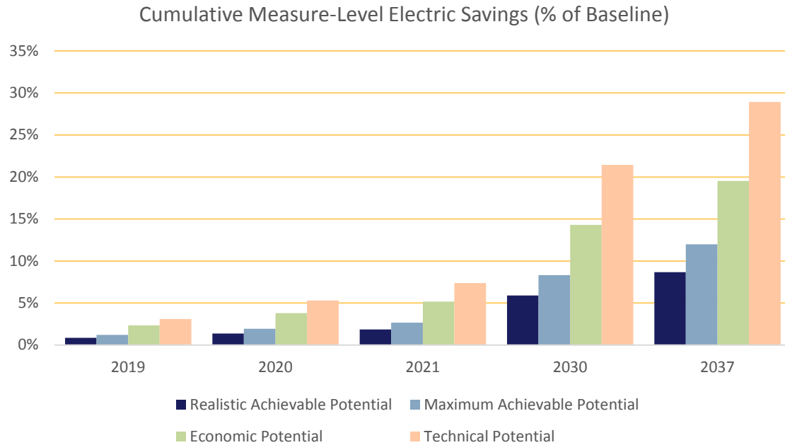
Figure 1-17 Summary of Cumulative Measure-Level EE Potential
