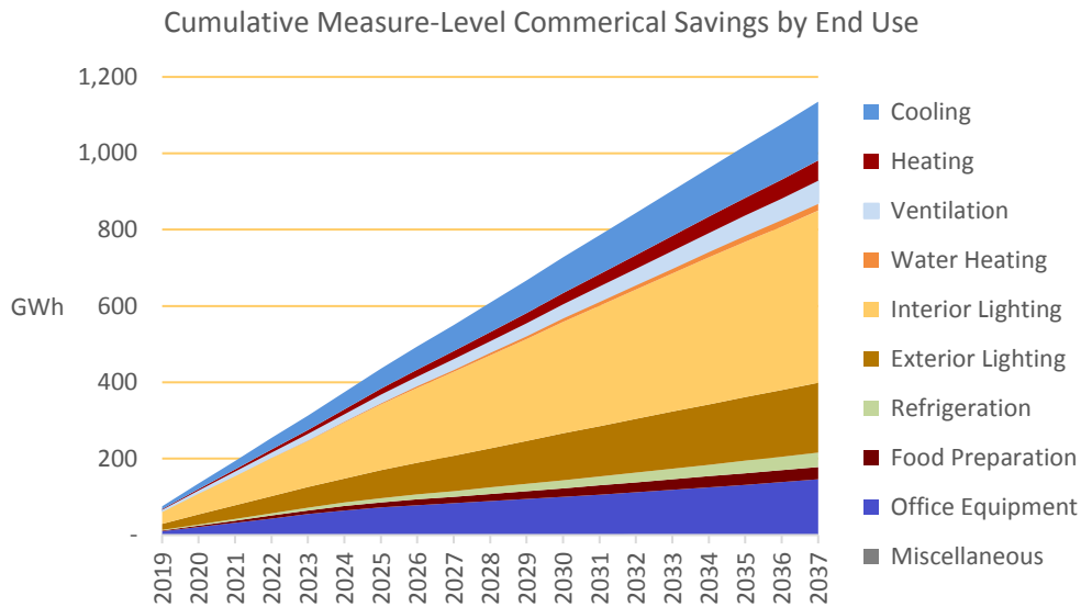
Figure 1-23 Commercial Sector Cumulative Savings (GWh) by End Use
