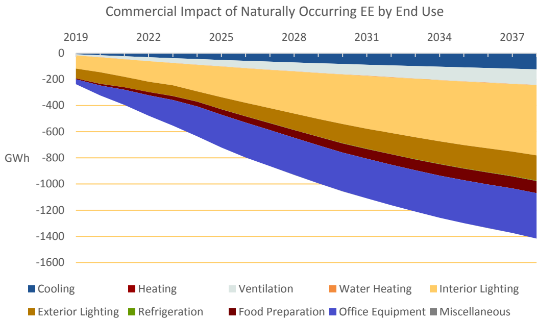
Figure 1-30 Commercial Impact of Naturally-occurring Energy Efficiency
