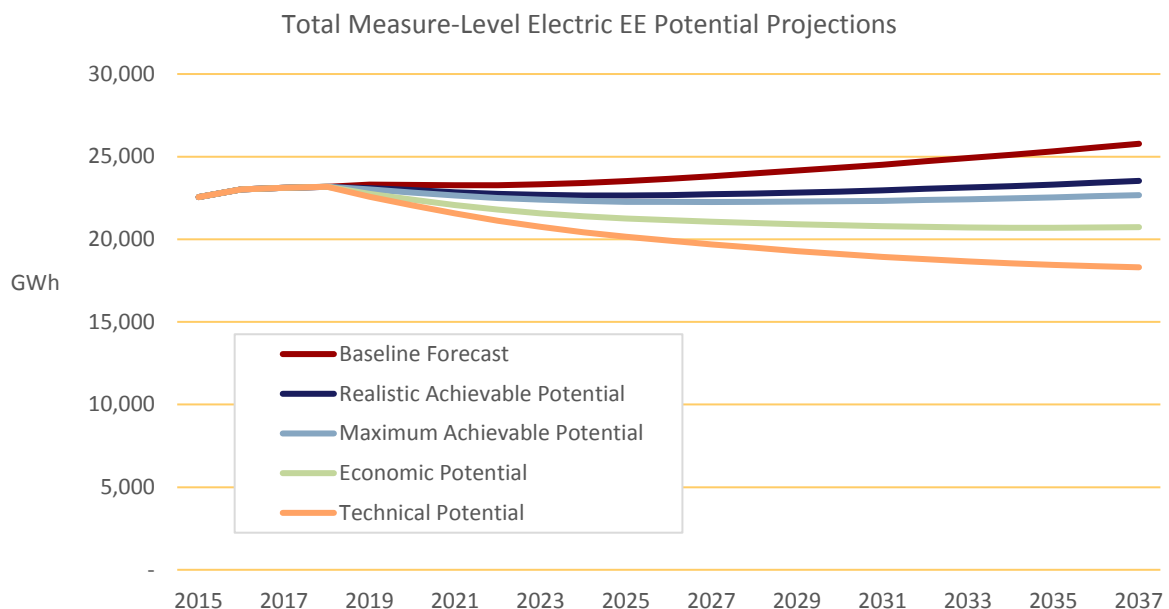
Figure 1-18 Summary of Baseline and Measure-Level EE Potential Projections
