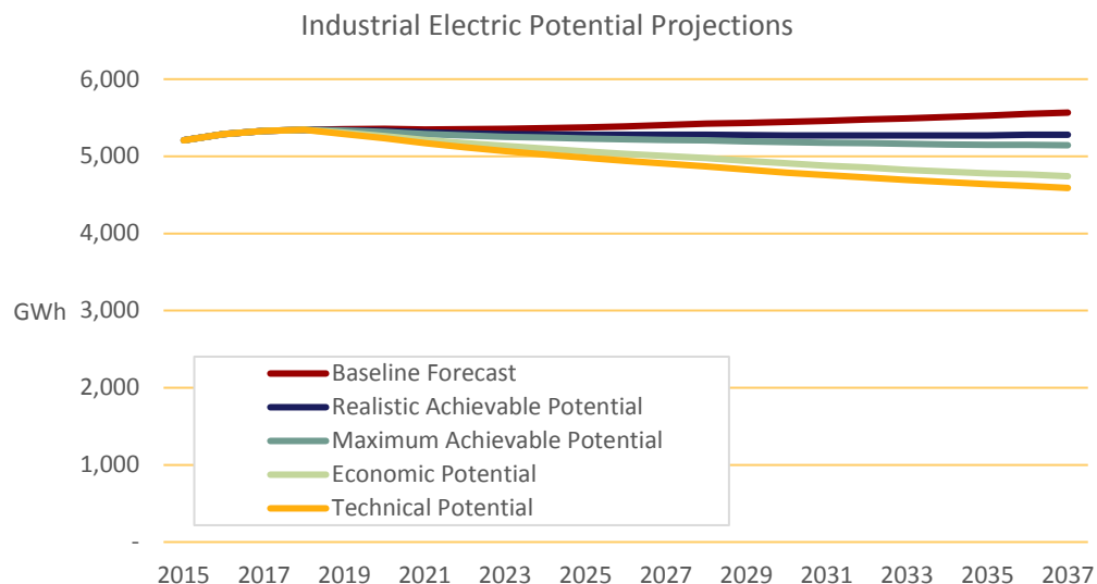
Figure 1-24 Industrial Sector EE Potential Projections
