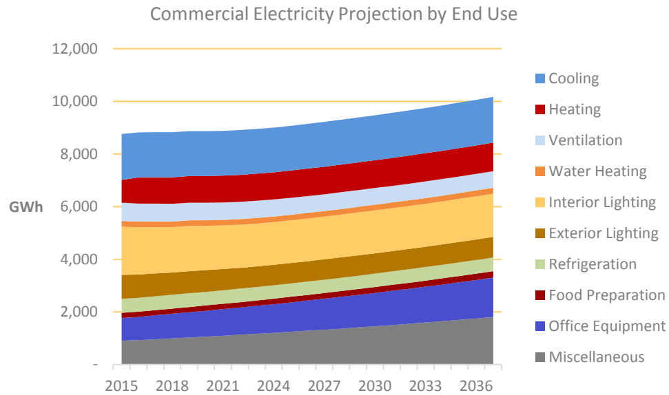
Figure 1-14 Commercial Baseline Electricity Projection by End Use
