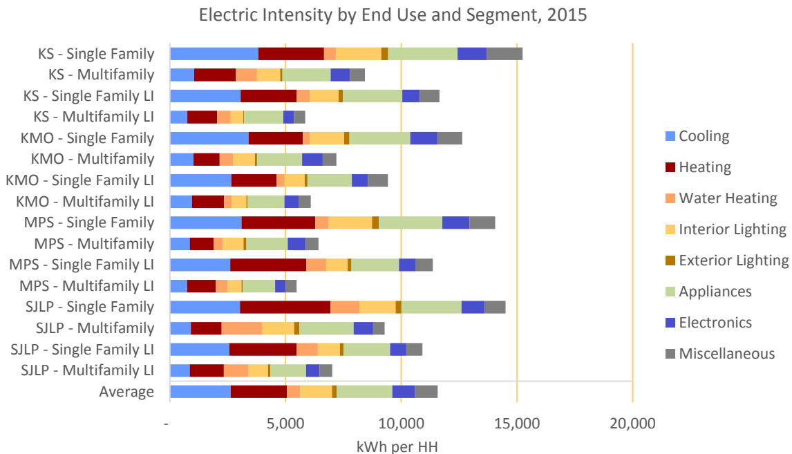
Figure 1-5 Residential Sector Electric Intensity by End use and Segment
