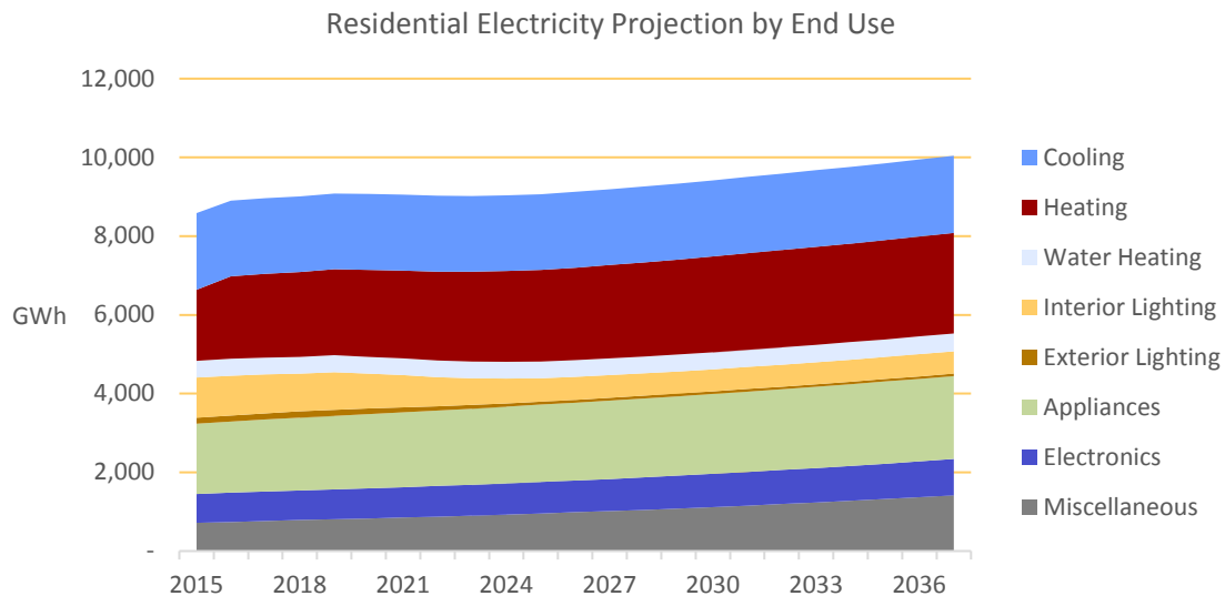
Figure 1-12 Residential Baseline Electricity Projection by End Use
