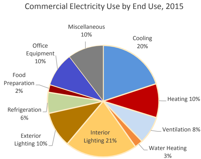
Figure 1-7 Commercial Energy Use by End Use
