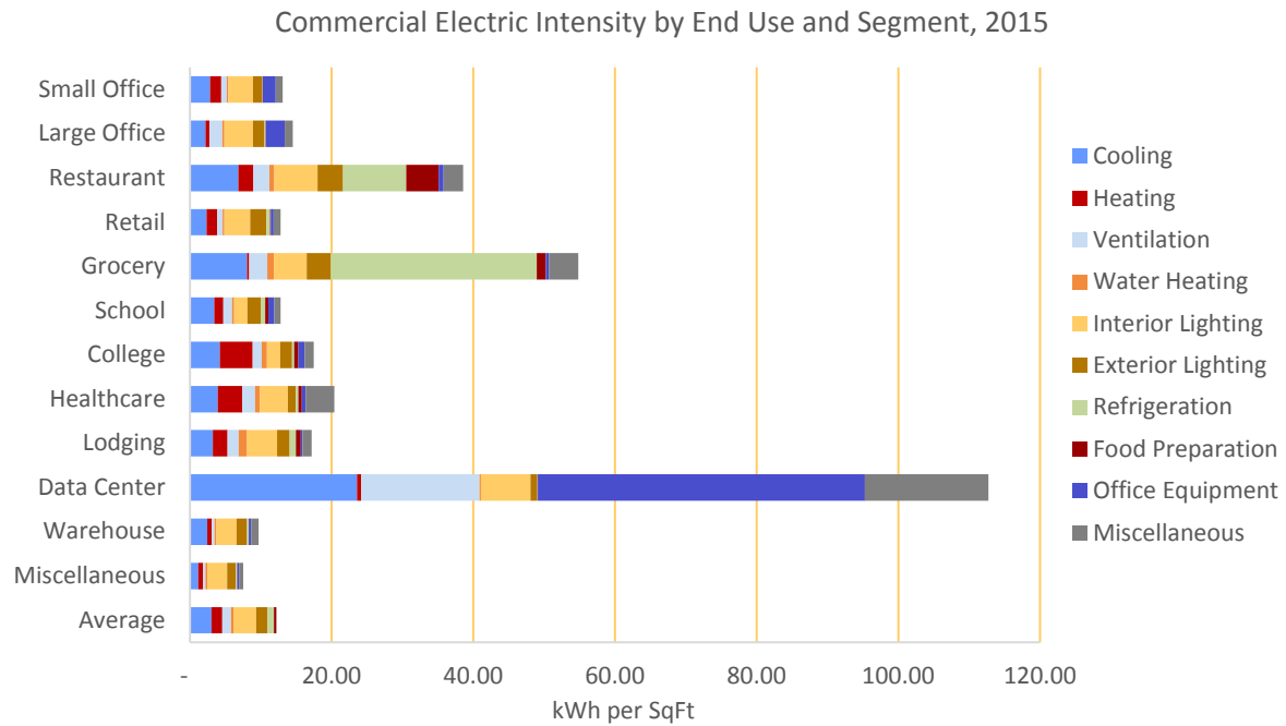
Figure 1-8 Commercial Electric Intensity
