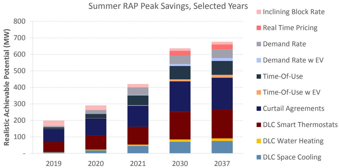
Figure 2-2 Realistic Achievable DR & DSR Potential (Summer MW)
