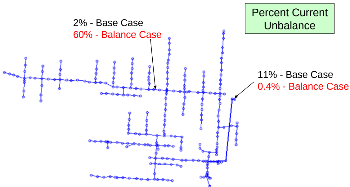
Figure 2-20: 3111 phase balance model percent unbalances in the circuit
