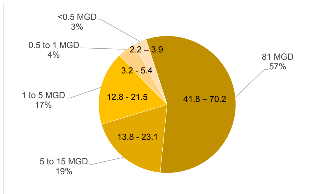
Figure 8. Wastewater treatment plant energy consumption by size category (GWh/year)
