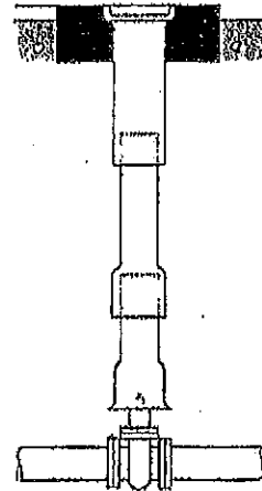
Profile View of Valve Box
