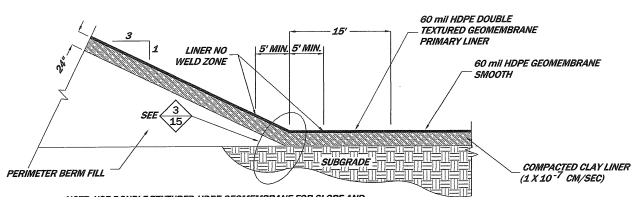
4 GEOMEMBRANE LINER TRANSITION DETAIL (TYP.)
