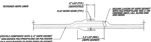
2 END-TO-END GEOCOMPOSITE CONNECTION
