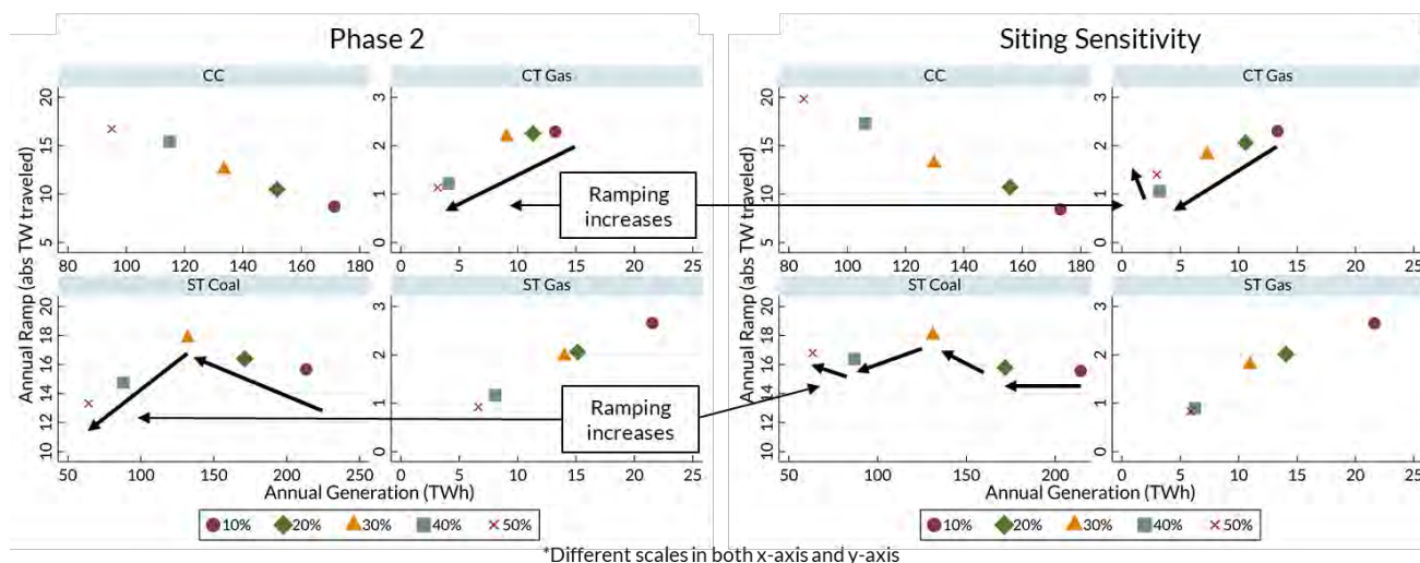
Figure EA-58: Thermal unit ramping for the siting sensitivity
