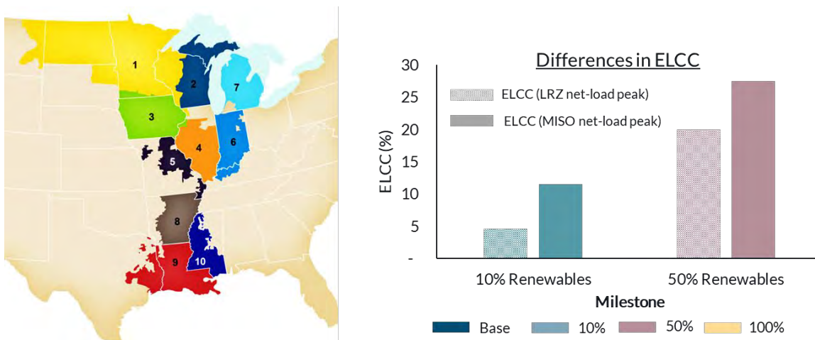
Figure RA-11: Change in ELCC by region size (MISO LRZ vs. MISO)
