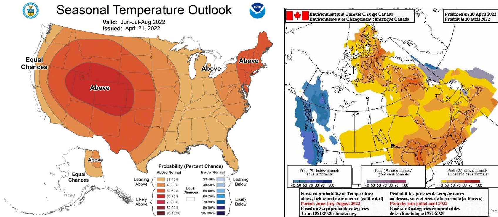
Figure 2: United States and Canada Summer Temperature Outlook 2
