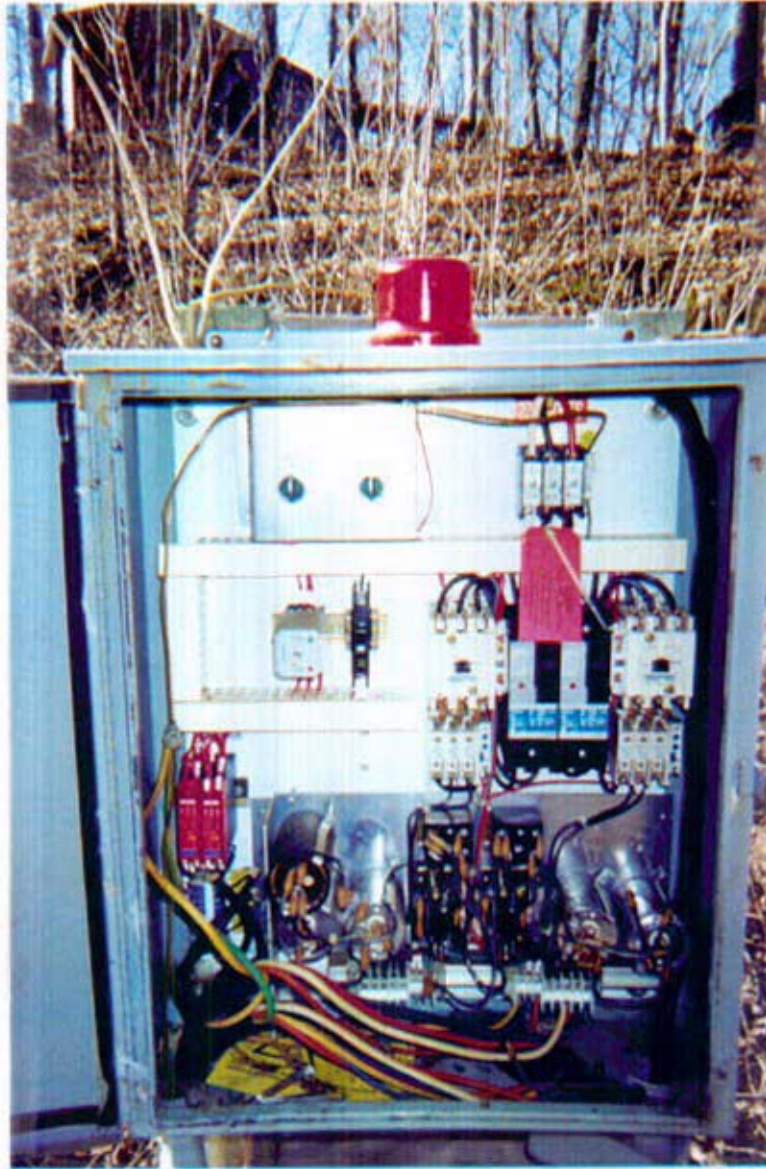
WARREN COUNTY WATER & SEWER – SHADY OAKS ELECTRIC PANEL AT LIFT STATION, SWITCHES OFF COMPONENTS MISSING 1/15/02
