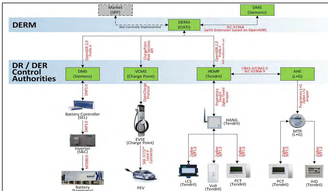
Figure 3-109: Implemented DR Integration Architecture
