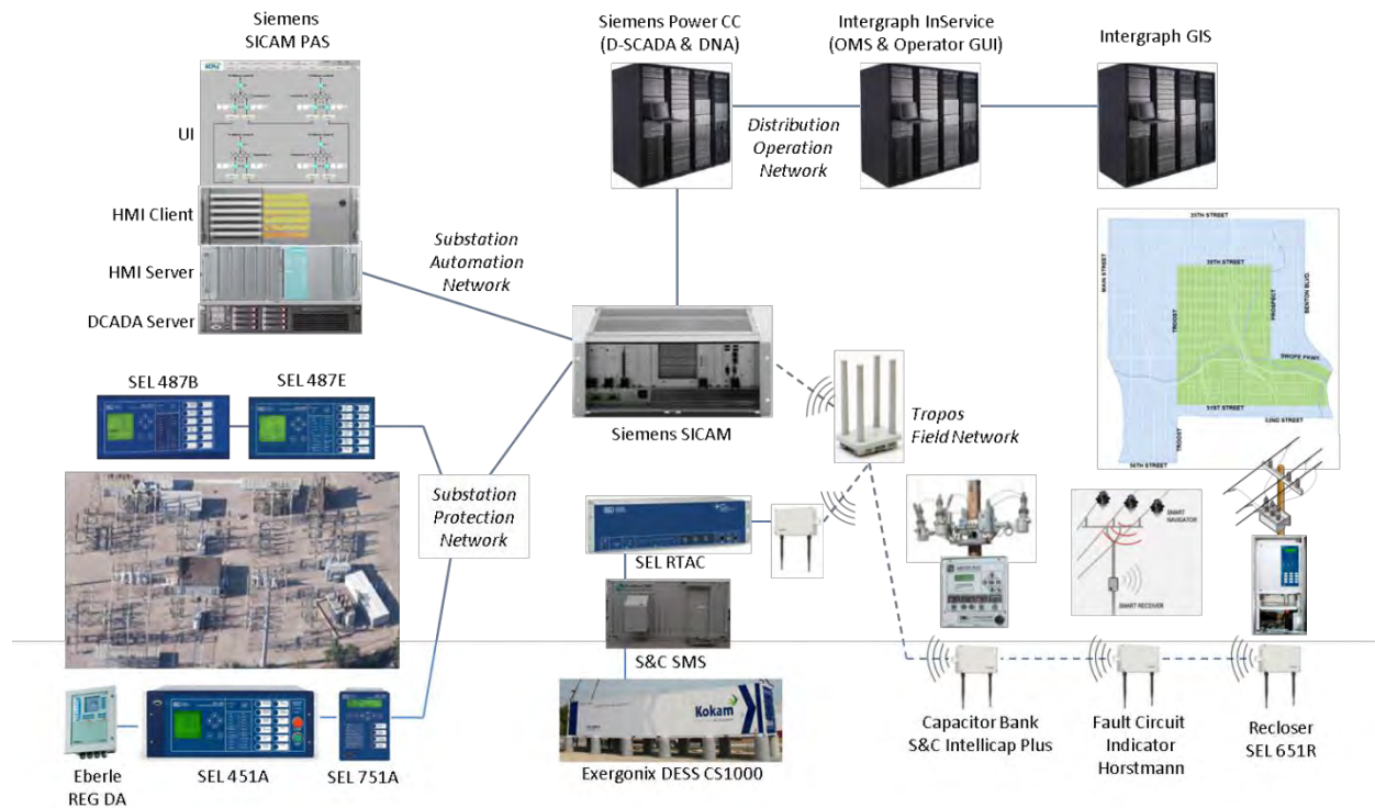
Figure 1-23: SmartDistribution Components
