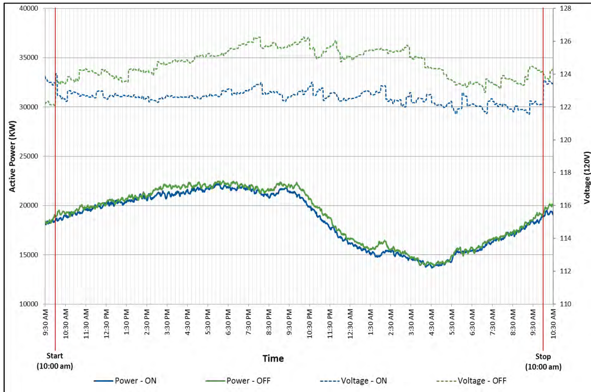
Figure 3-39: TF #7/8 Active Power & Voltage Comparison (07/15–07/16)
