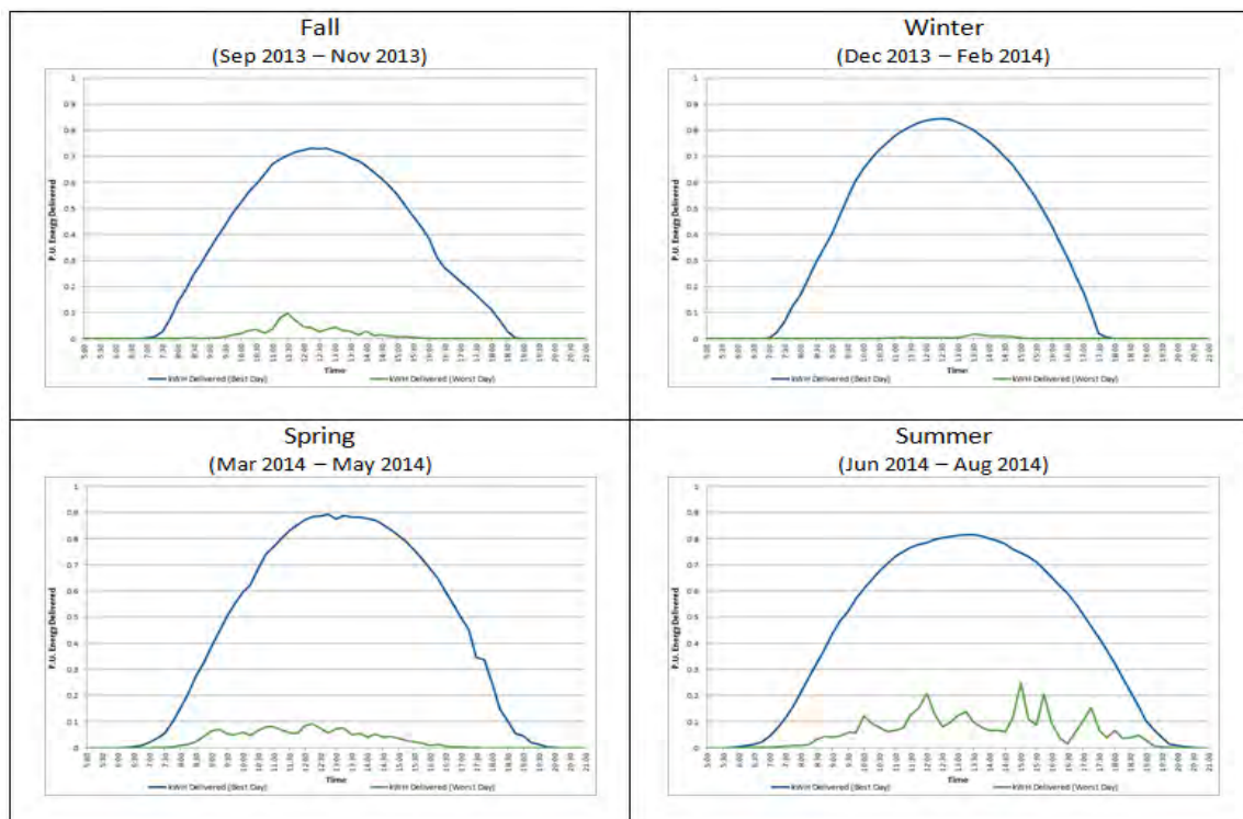
Figure 3-145: Composite Solar kW – Typical Day
