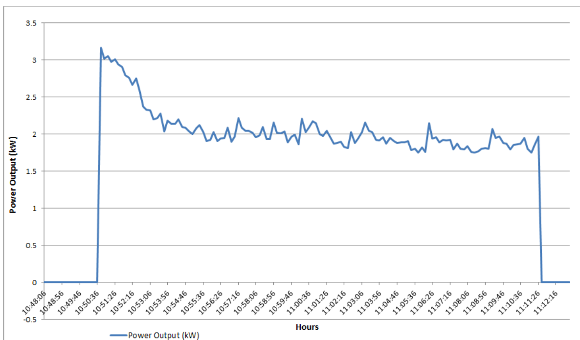
Figure 3-76: Battery and SMS Load Graph During Islanding
