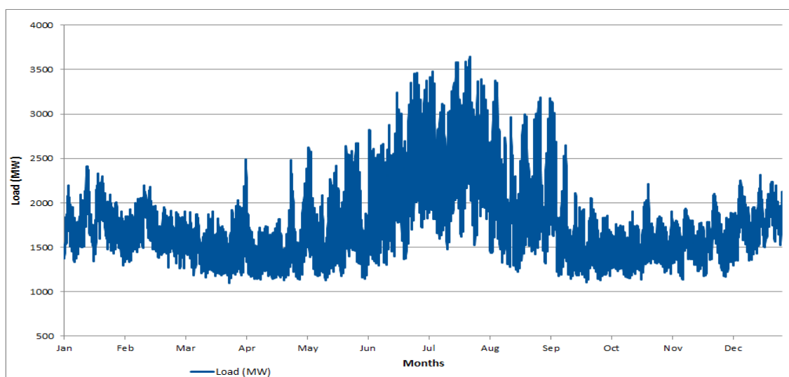
Figure 3-161: KCP&L 2012 System Hourly Load Profile
