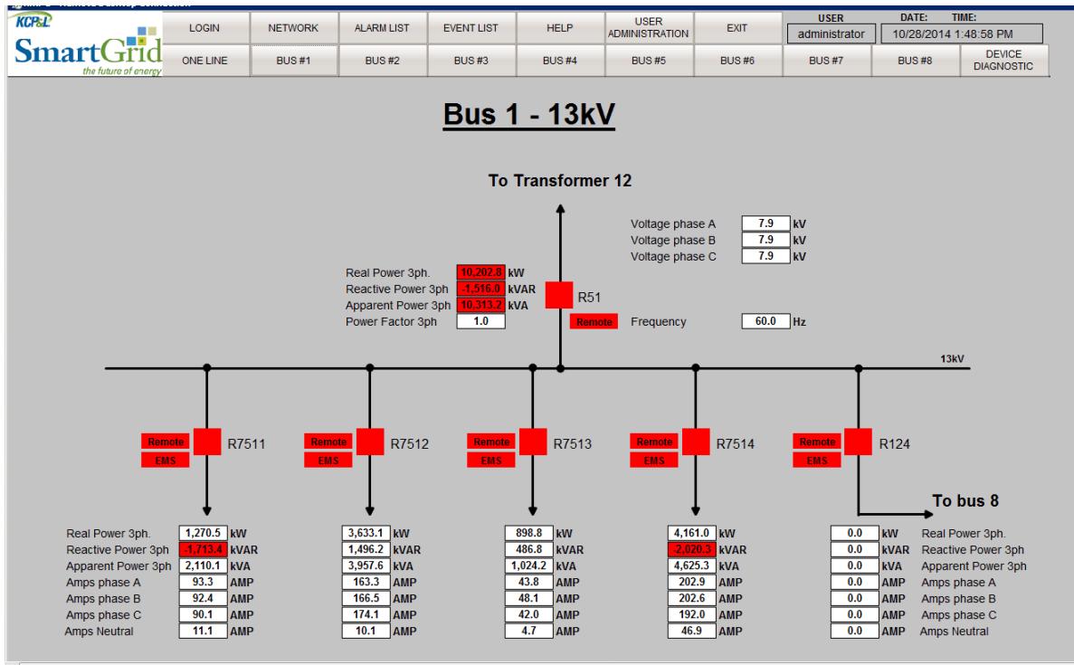
Figure 3-84: HMI Single-Bus View
