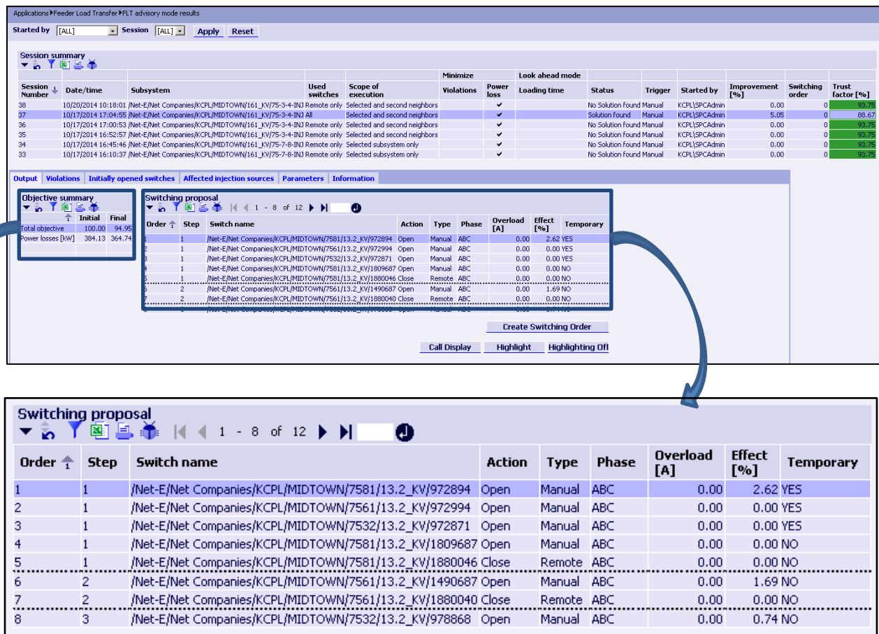
Figure 3-54: Result – Minimize Losses with Automated and Manual Switches #1
