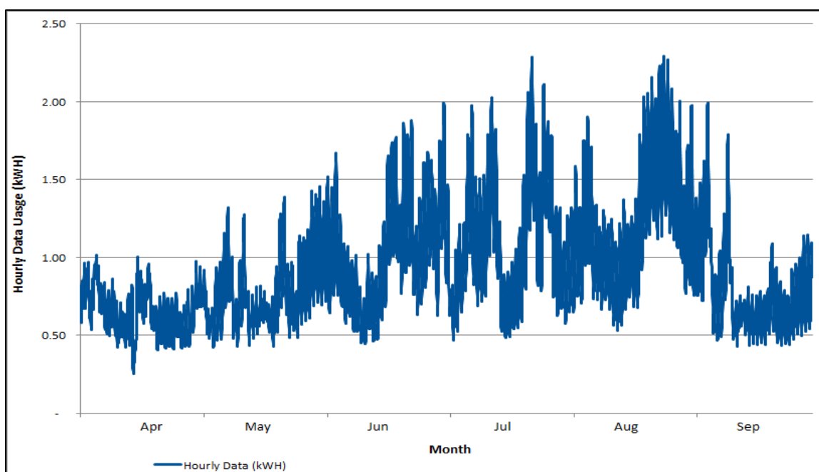
Figure 3-99: SmartGrid Residential Rate Class Load Profile (April–September 2014)
