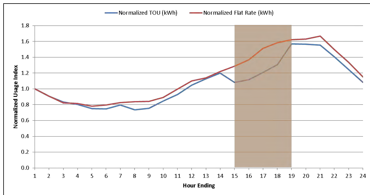
Figure 3-132: Initial TOU Usage Impact Analysis
