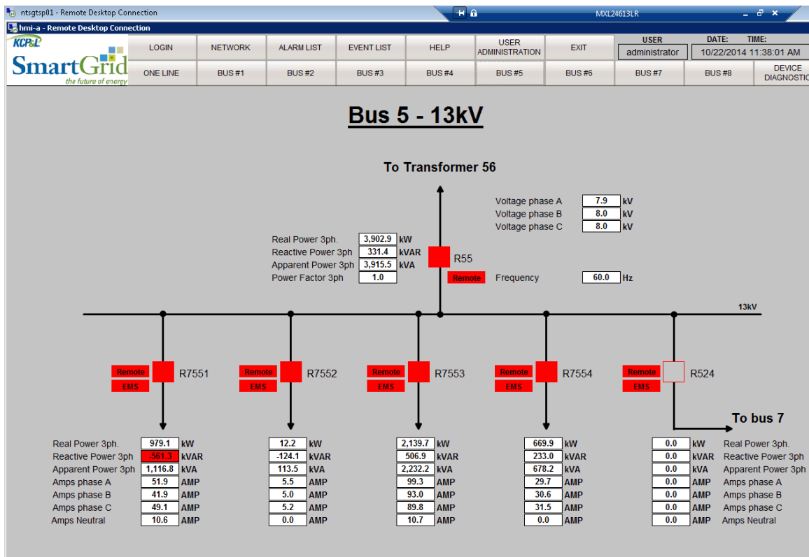
Figure 3-80: Example HMI Data Presentment
