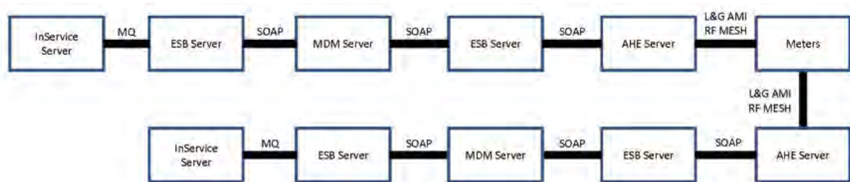
Figure 3-106: Systems Integration Supporting Power Status Verification Functions
