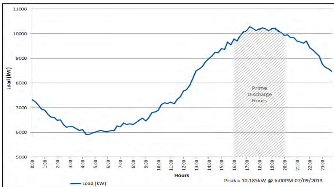
Figure 3-175: 2013 Peak Day Load Profile Circuit 7571
