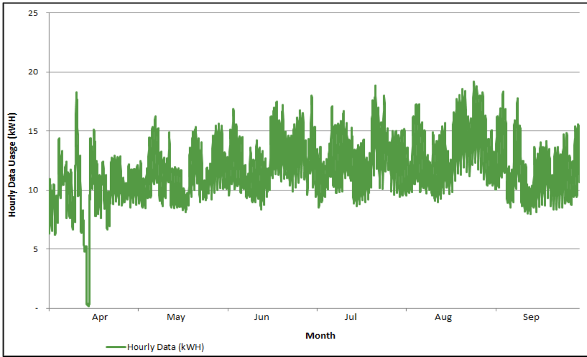
Figure 3-101: SmartGrid Commercial Rate Class Load Profile (April–September 2014)
