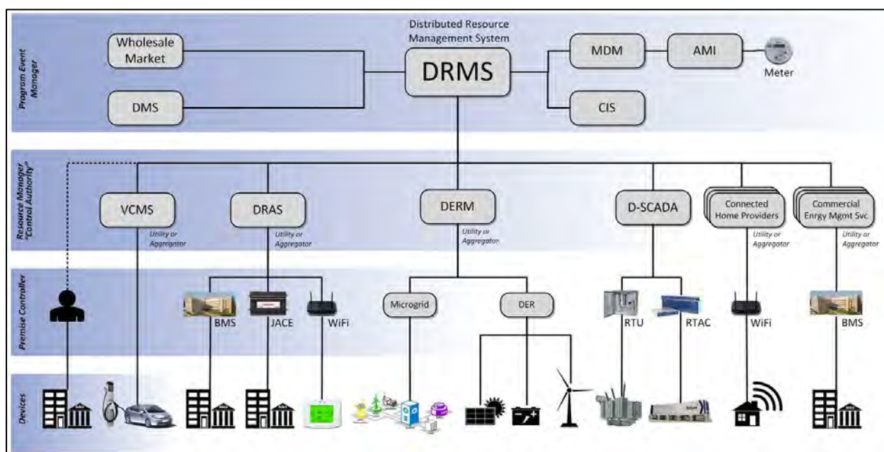
Figure 3: DRMS Proposed Architecture
