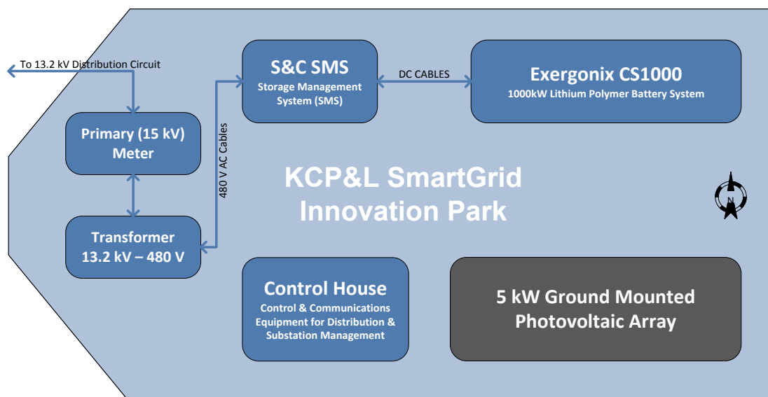
Figure 3-26: KCP&L's Smart Grid Innovation Park Site Layout
