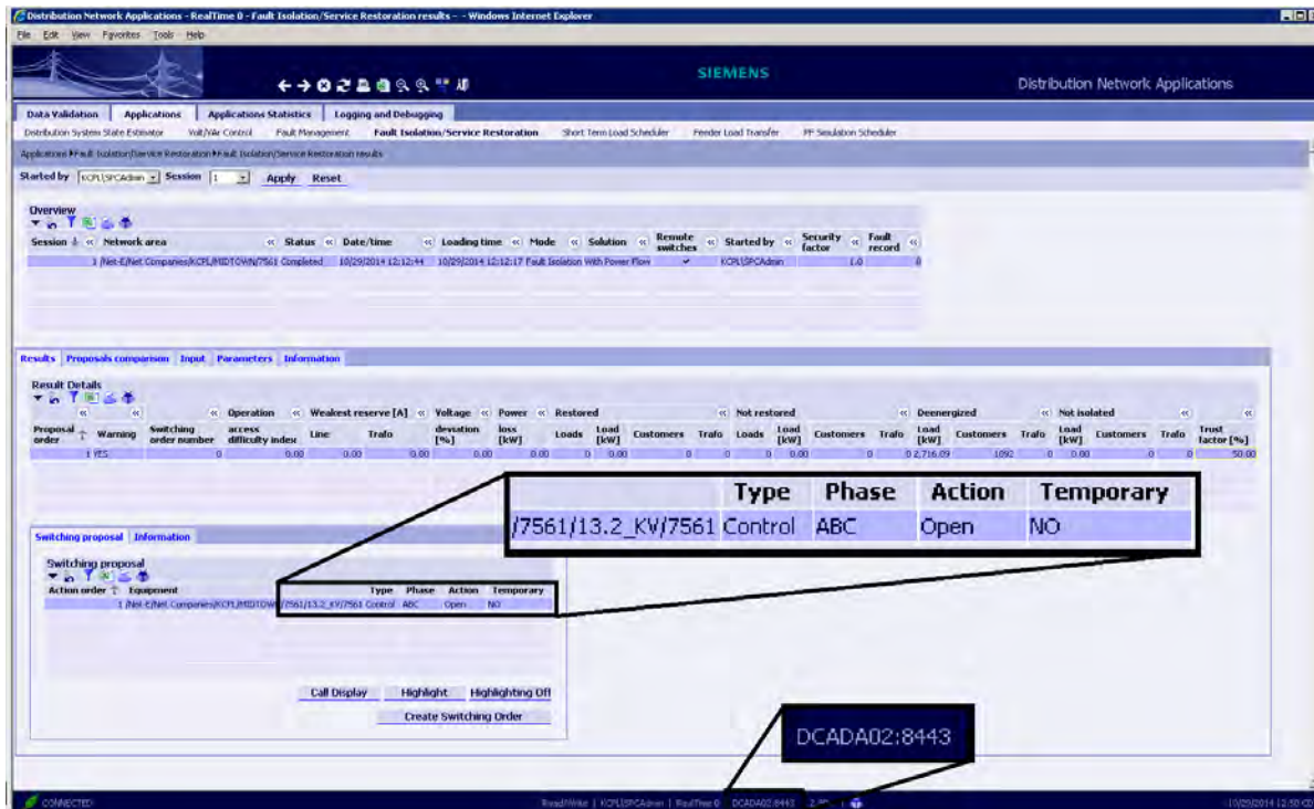
Figure 3-96: FISR via the DCADA
