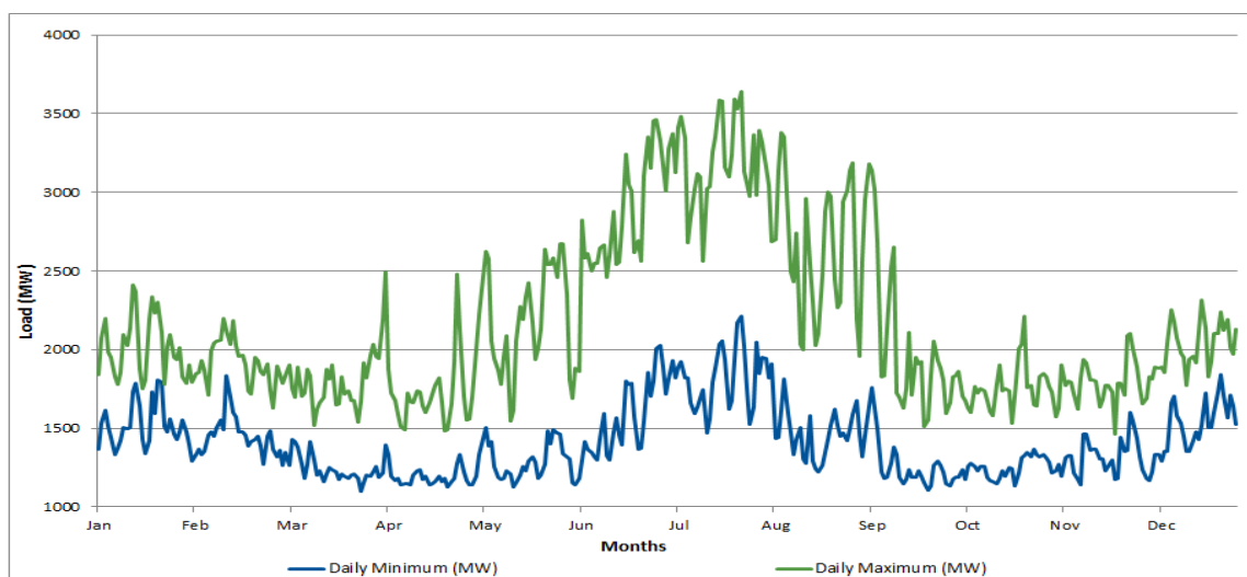
Figure 3-162: 2012 Daily System Minimum and Maximum Loads
