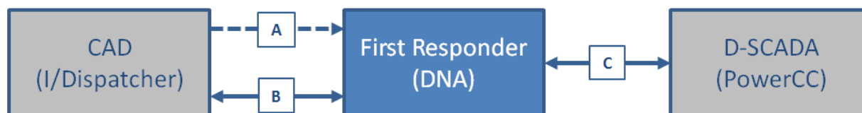
Figure 2-58: KCP&L SmartGrid Demonstration Project First Responder Integration
