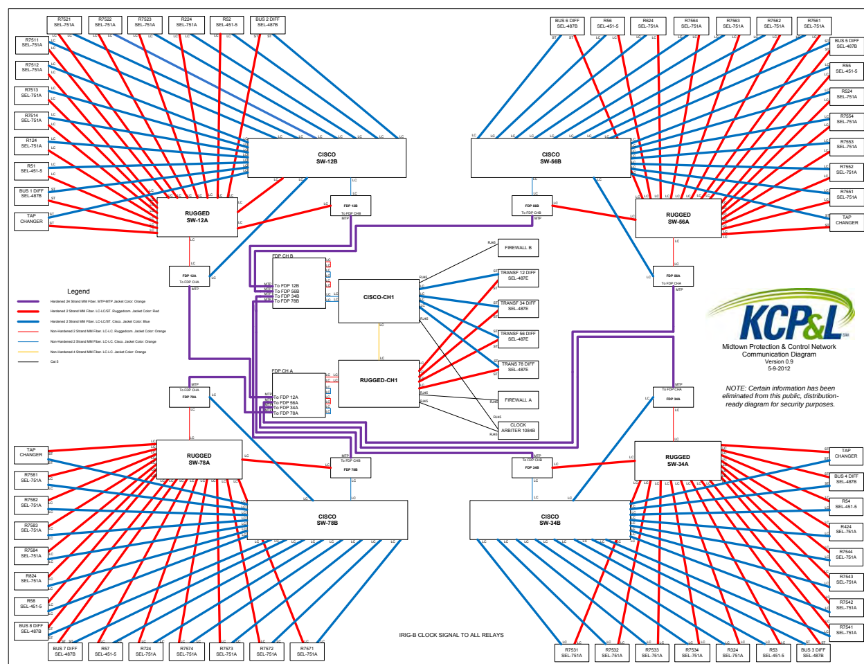
Figure 2-83: Midtown Substation
