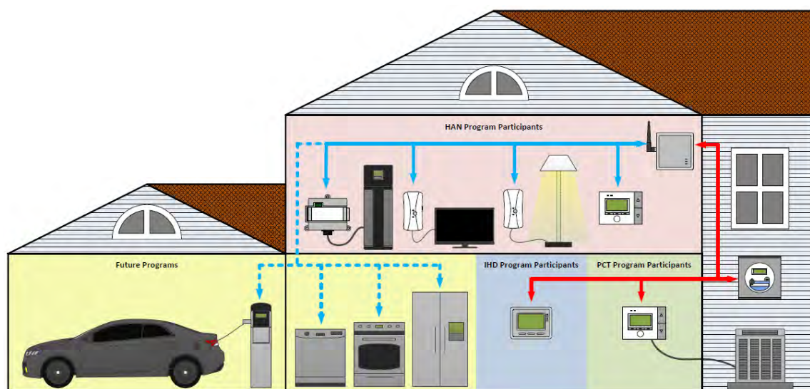
Figure 2-85: SmartEnd-Use Home Configuration
