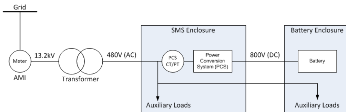
Figure 3-147: Battery-Inverter Interconnection
