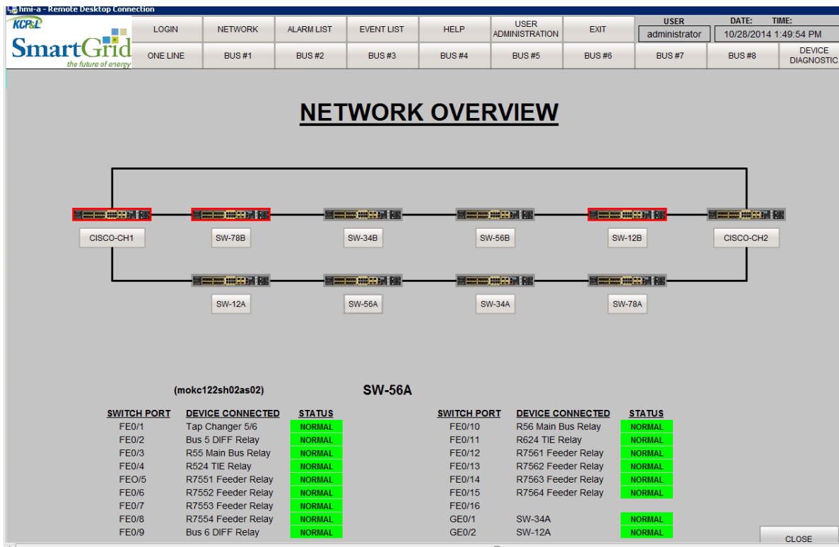
Figure 3-85: HMI Network Overview
