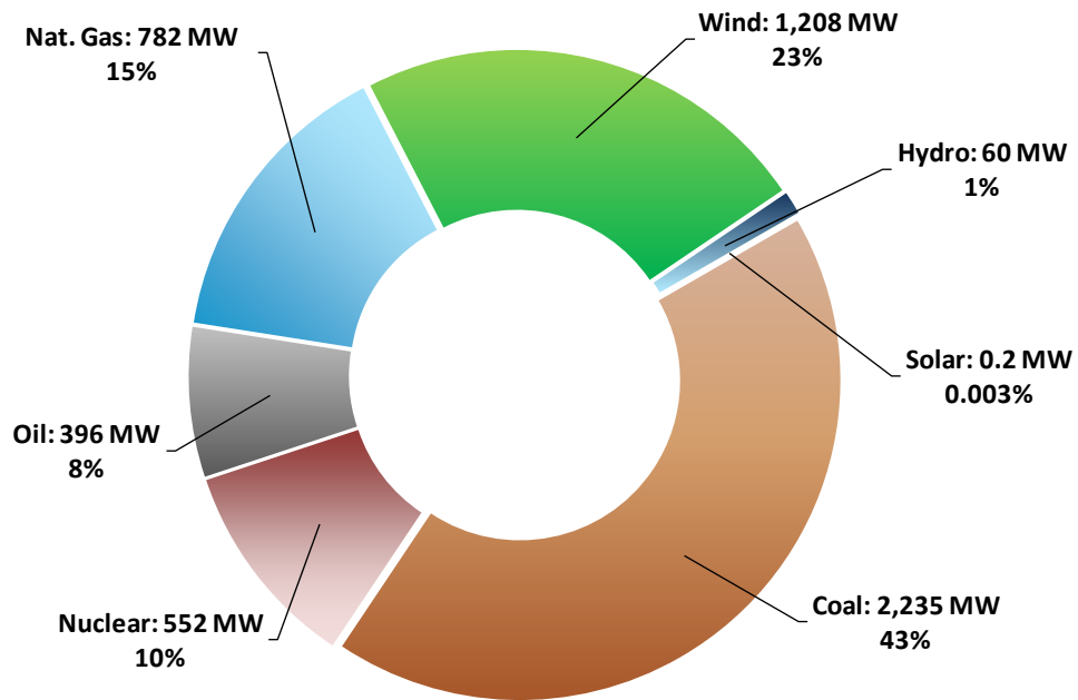
Figure 2: Capacity By Resource Type
