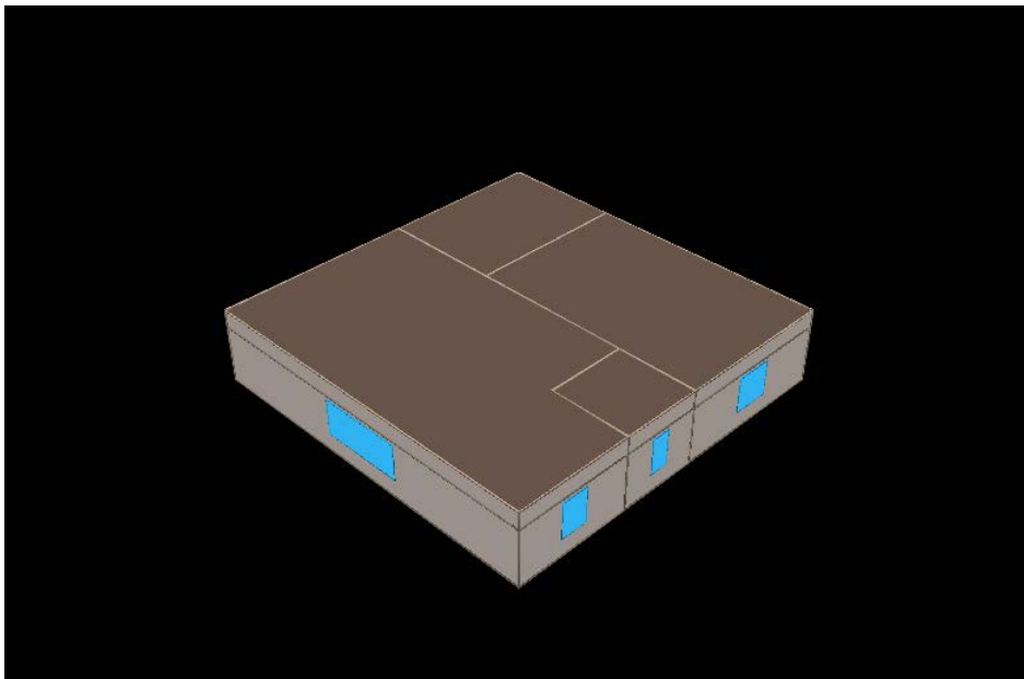
Figure 6. Full Service Restaurant Prototype Rendering
