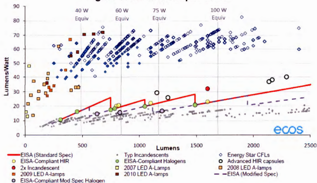
Figure 7. 32: EISA Implications
