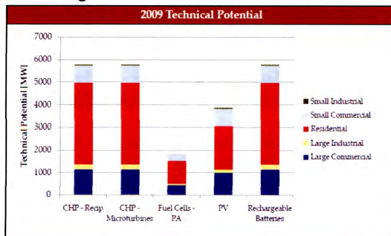
Figure 7. 15: DG Technical Potential
