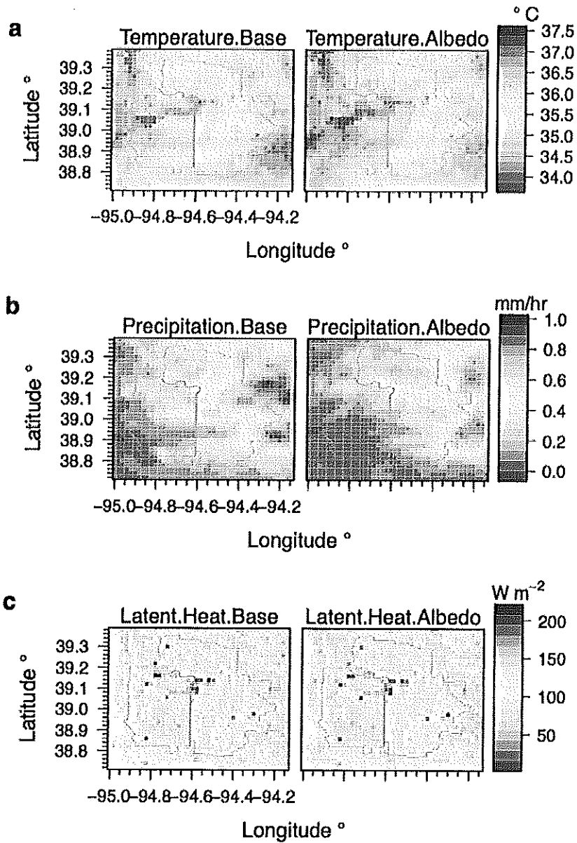
Figures 6. Comparison of early evening (15:00 – 19:00 LST) mean air temperature (a), non-convective precipitation (b) and latent heat (c) between the control case and the roof albedo scenario during the heat wave episodes. “base” and “albedo” denotes the control and cool roof albedo cases, respectively.
