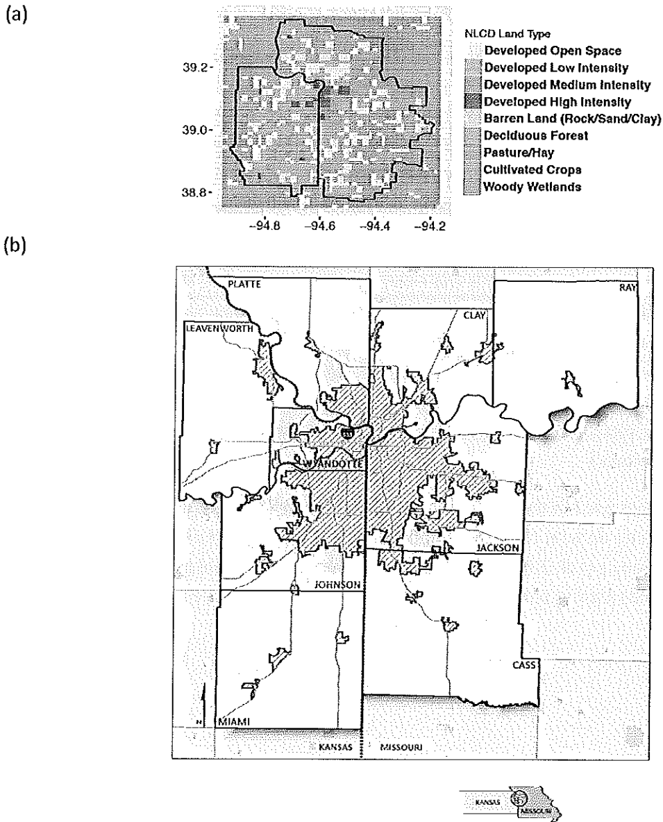
Figure 4. Maps of the urban areas as used in (a) the meteorological simulations (jagged black line is the outline of the urban areas) and (b) the power calculations (cross-hatched areas are urban).
