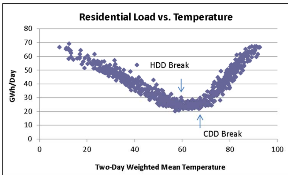
Figure 3.9: Residential Load/Temperature Relationship
