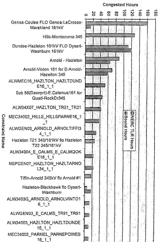
Sorted by Greater of: TLR or Bound Hours Top 19 Elements (Congested More Than 1% of Time) 4/1/2005 through 3/31/2006
