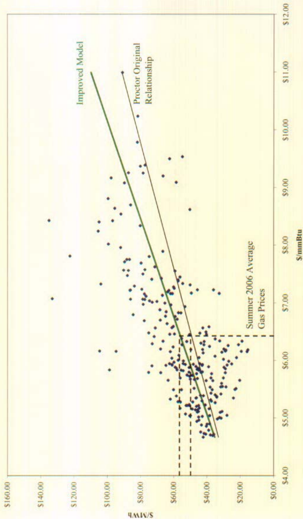
Dr. Proctor's Original On-Peak Relationship Compared to Improved Model with Corrected and Updated Daily Data (Summer Months)
