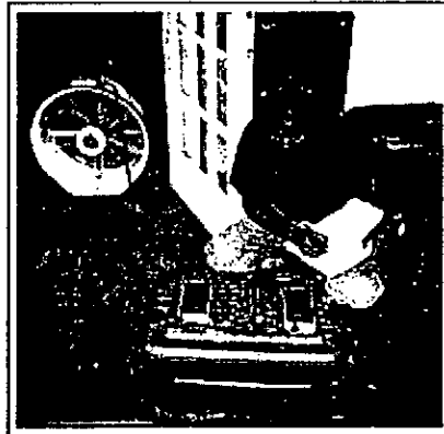
The blower door and pressure-measuring gauges are useful both in quantifying duct leakage associated with duct work and in revealing the locus of significant leaks. Protocols for using both blower doors and the distribution system's own fan to quantify leaks are currently being developed, and several companies have recently developed small calibrated blowers useful in leak detection and quality control in duct sealing.
