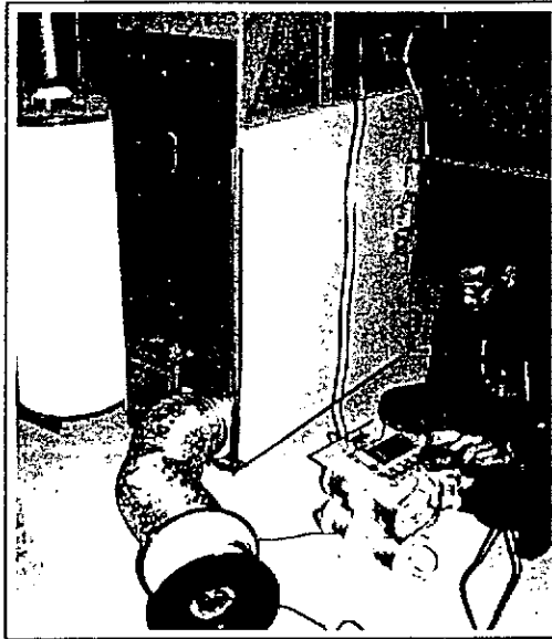
The blower door and pressure-measuring gauges are useful both in quantifying duct leakage associated with duct work and in revealing the locus of significant leaks. Protocols for using both blower doors and the distribution system's own fan to quantify leaks are currently being developed, and several companies have recently developed small calibrated blowers useful in leak detection and quality control in duct sealing.
