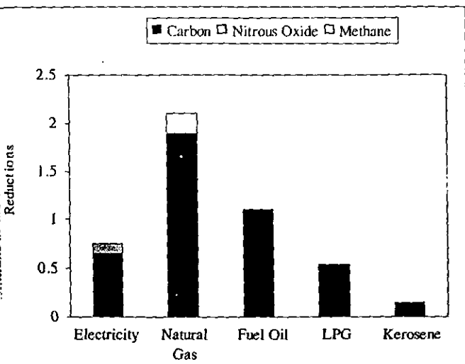
Annual change equivalent emission reductions of all houses weatherized by the program in 1989 over the 20-year lifetime of measures, by type of heating fuel
