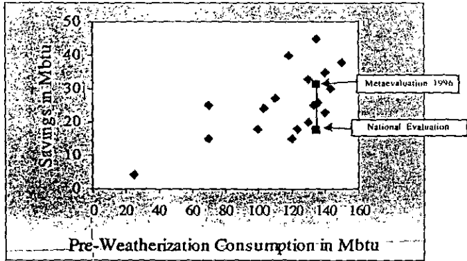
At Same Levels of Pre-Weatherization Consumption, Most Evaluations Completed Since 1990 Show Higher Savings Than in 1989
