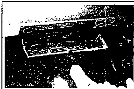
Permanent air sealing of the return air system is accomplished with a fiberglass mesh and special mastic.
