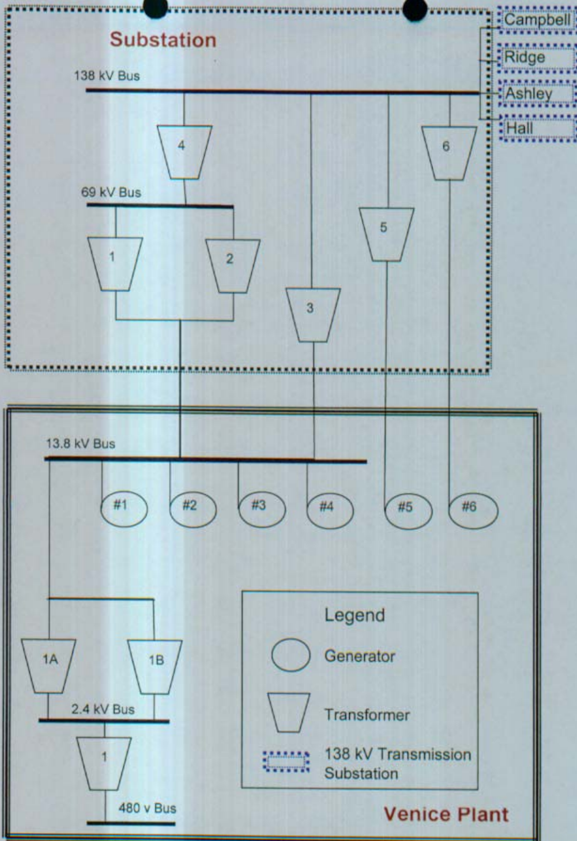
Simple electrical diagram of Venice Plant and Venice Substation.
