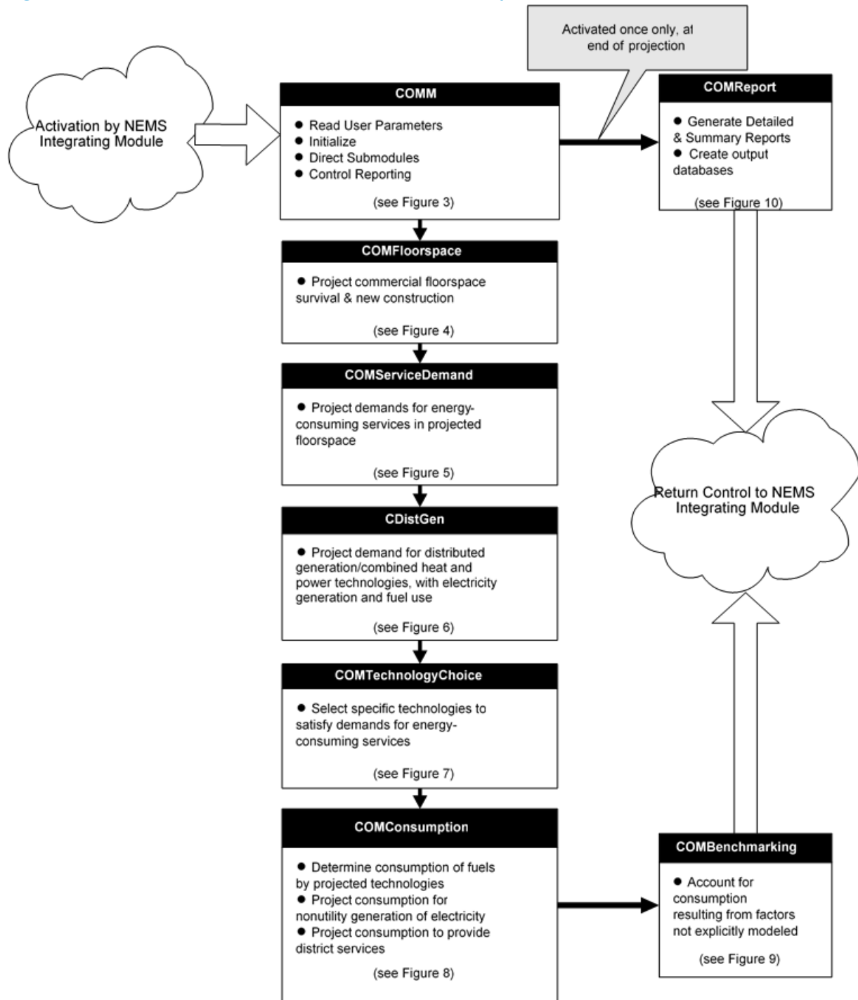
Figure 2. Commercial Module structure and fundamental process flow
