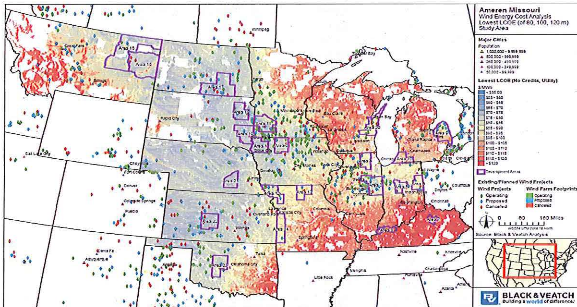
Figure 6.7 Wind Analysis Identified Development Areas and LCOE
