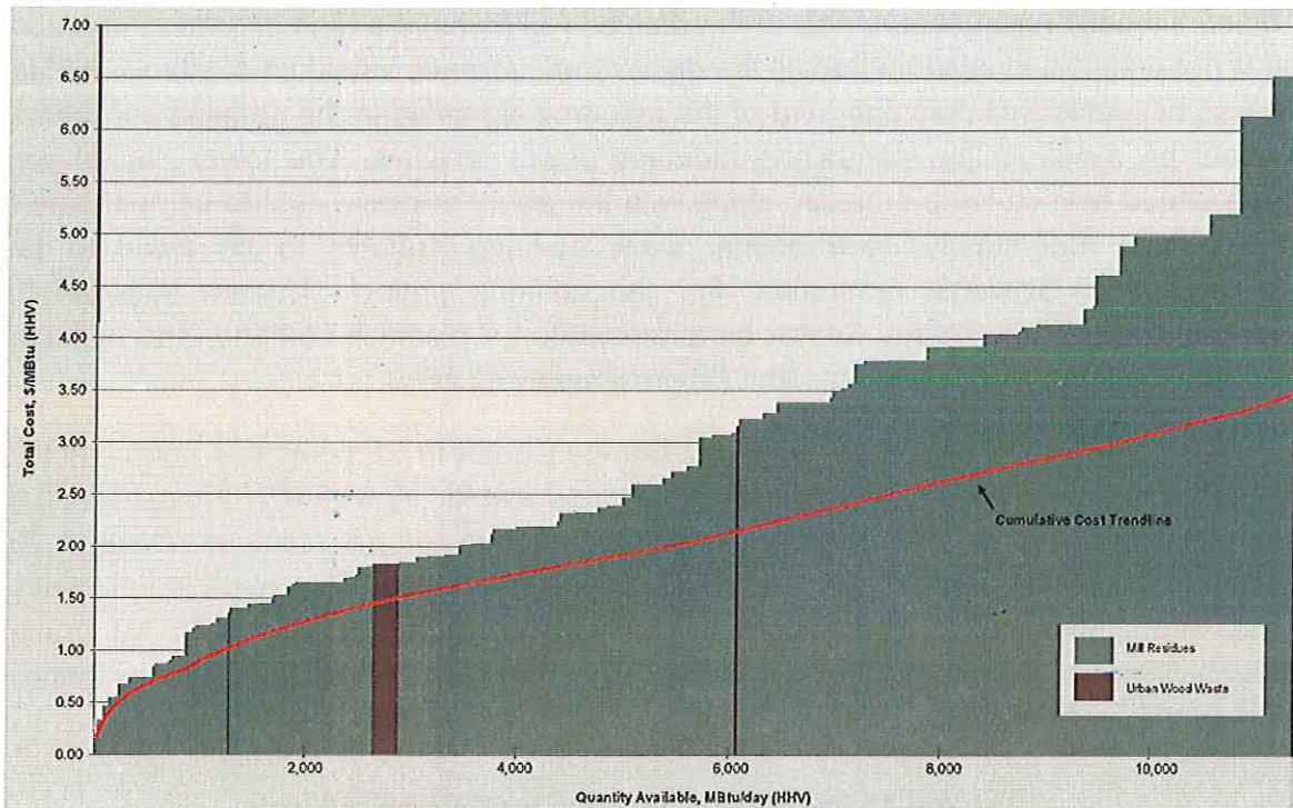
Figure 6.3 Biomass Fuel Supply Curve for Ellington Region
