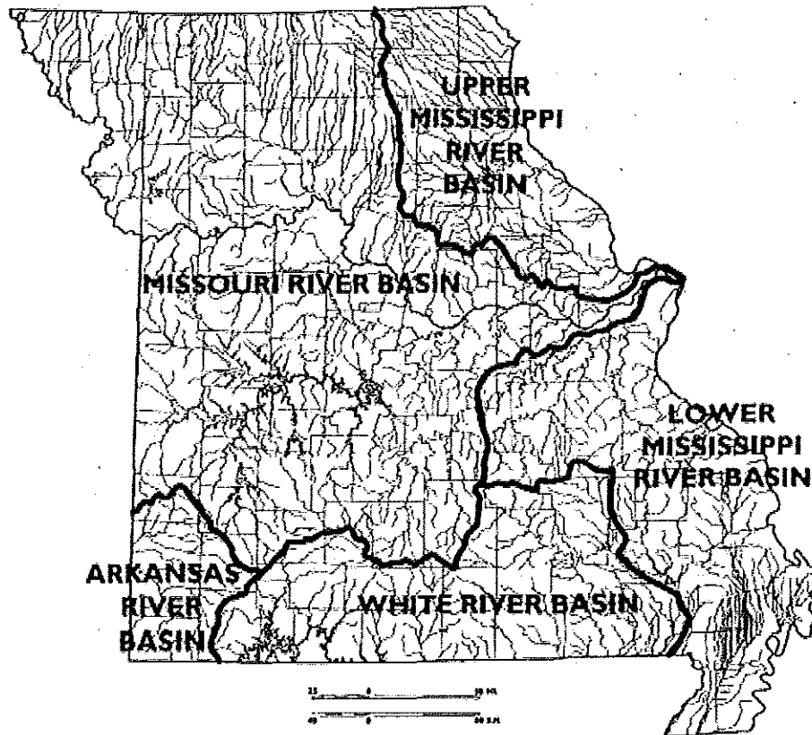
5 Figure 5: Major drainage basins in Missouri 19
