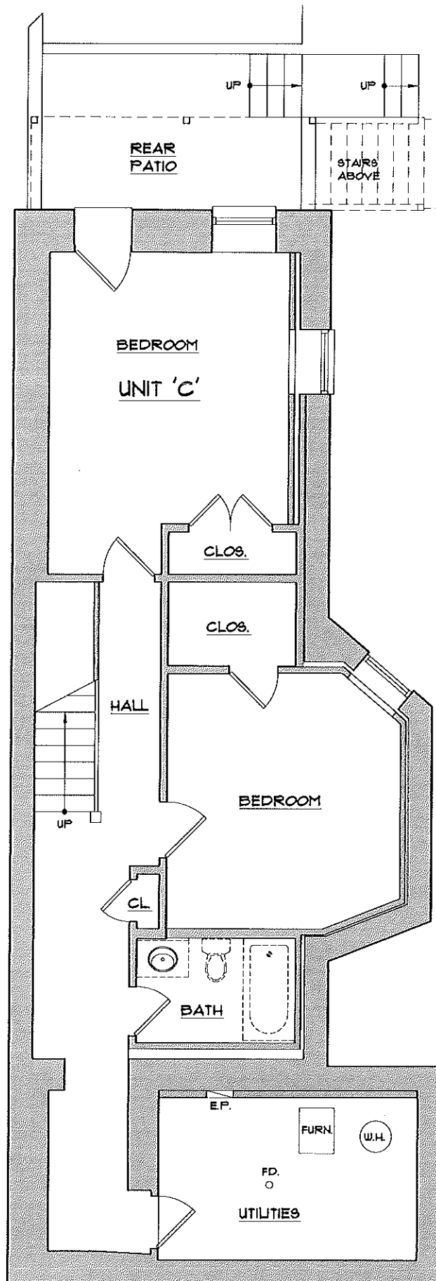
1 UNIT 'C' LOWER LEVEL 1/4" = 1'-0"
