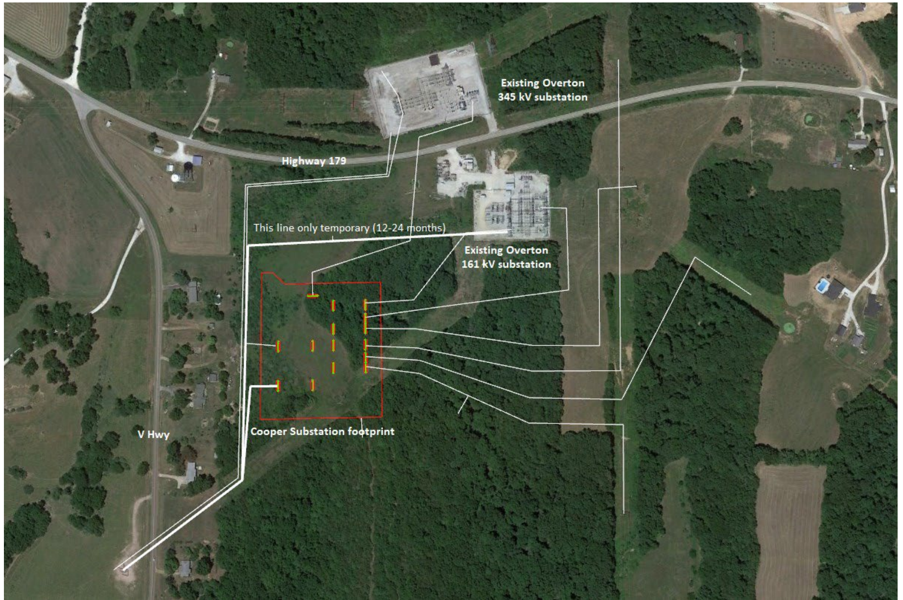
Figure 2 – Overview of Cooper Substation Footprint and Associated Transmission Lines
