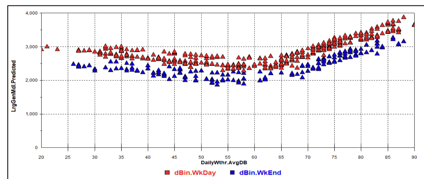
Predicted vs Daily Average Temperature
