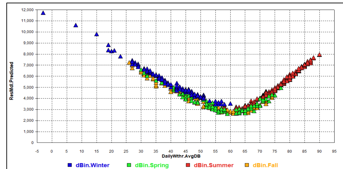
Predicted vs Daily Average Temperature
