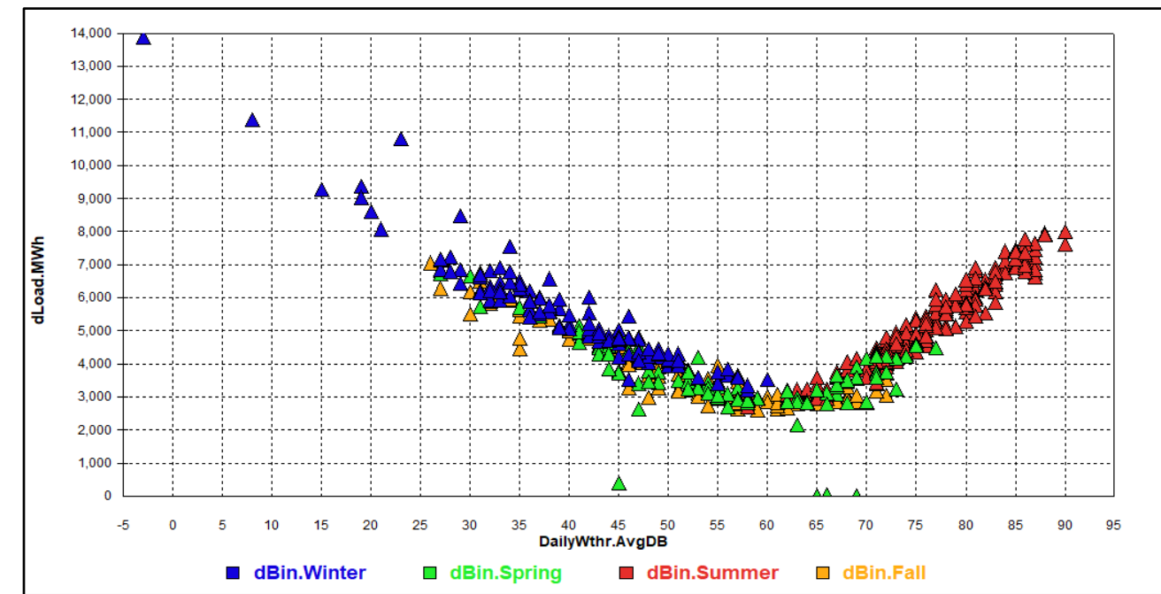
Actual vs Daily Average Temperature
