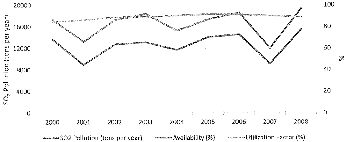
Unit 1 SO 2 Pollution Tracks Availability, Not Demand on the Unit
