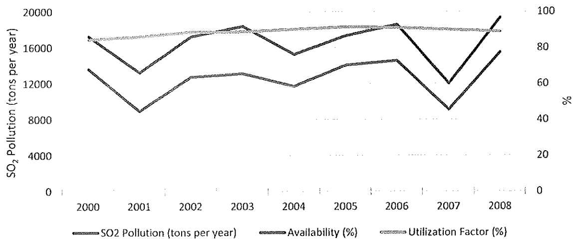
Unit 2 SO 2 Pollution Tracks Availability, Not Demand on the Unit
