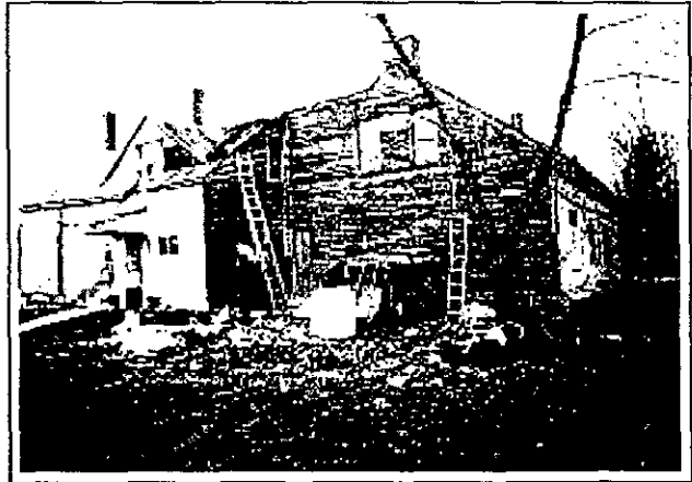
Movement of deteriorated foundation walls has opened large paths for air leakage.
