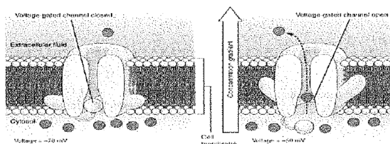
Figure 28 Voltage Gated Calcium Channels
