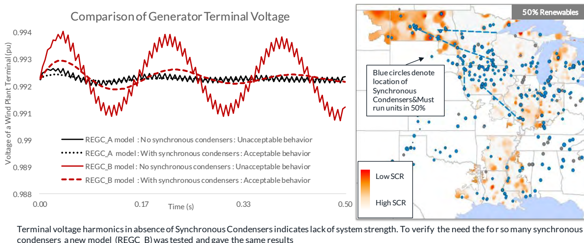
Figure OR-DS-10: At 50% milestone system-wide installation of synchronous condensers may be required
