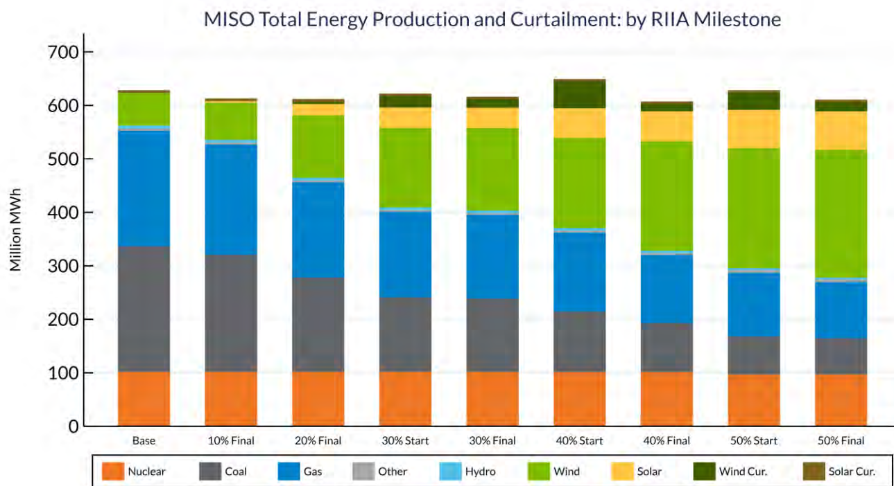
Figure EA-1: Fuel mix in RIIA milestones. “Start” indicates the addition of all renewables for the current milestone, plus any incremental transmission improvements from the previous milestone. “Final” indicates the addition of all renewables and any incremental improvements for the current milestone. The 30% model required transmission upgrades to meet OR performance requirements.
