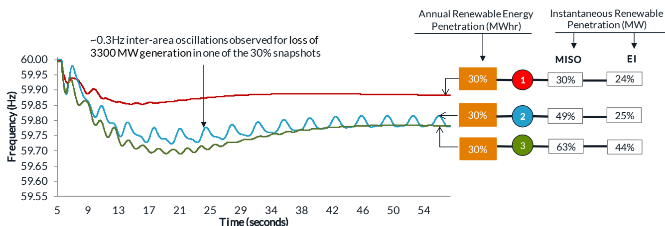
Figure OR-DS-23: Inter-area small signal stability issues observed in low-load high renewable in 30% milestone
