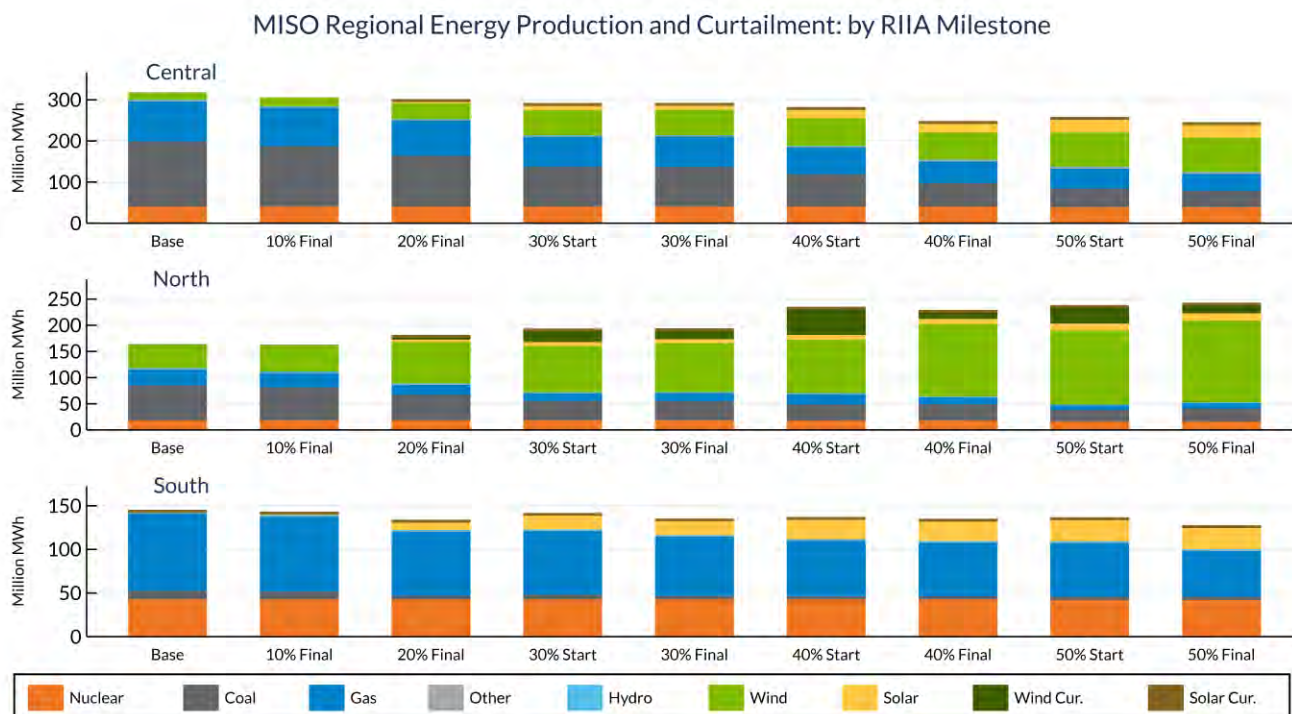
Figure EA-3: Fuel mix in RIIA milestones, regional breakdown
