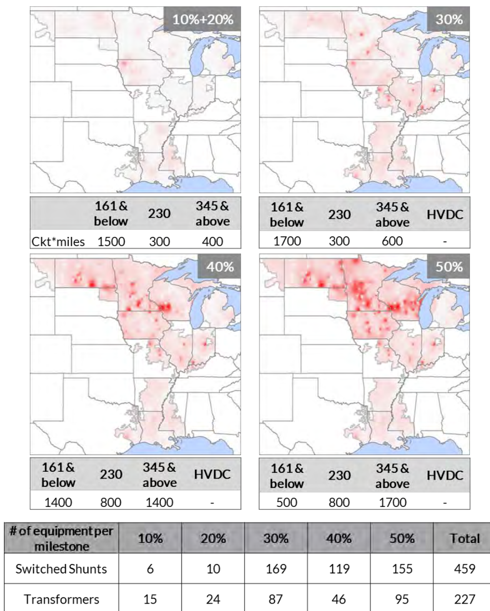
Figure UC-9: Steady state - cumulative complexity at renewable penetration milestones
