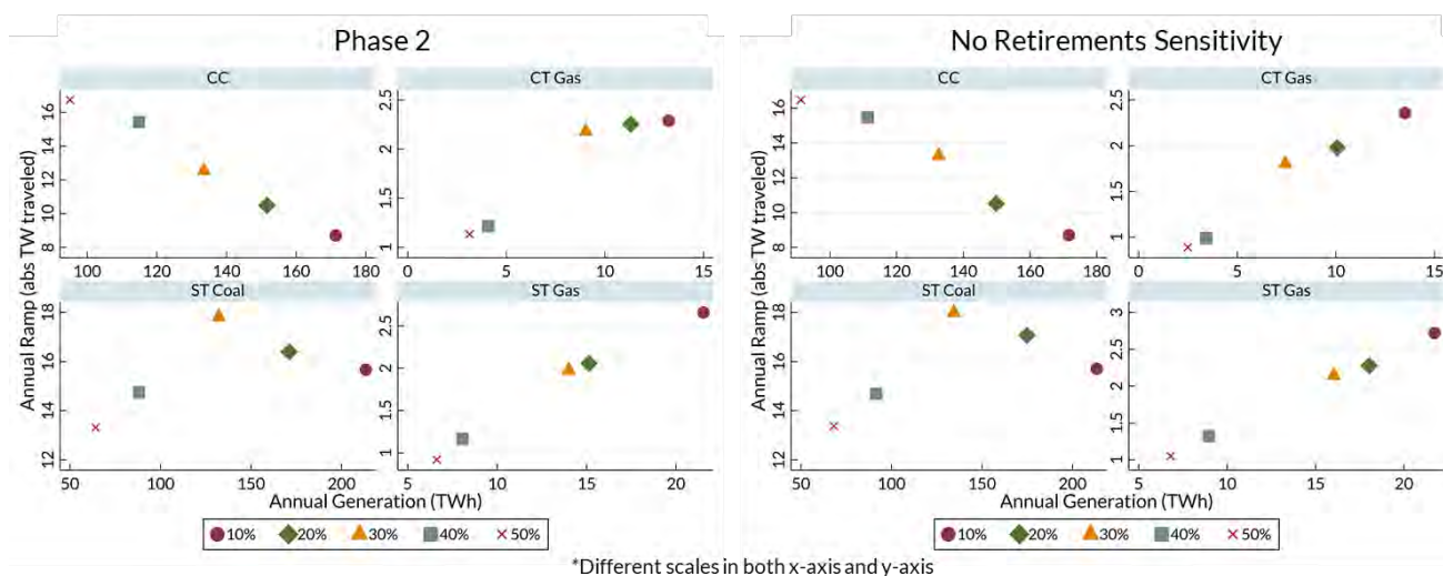
Figure EA-50: Thermal unit ramping in the no retirements sensitivity
