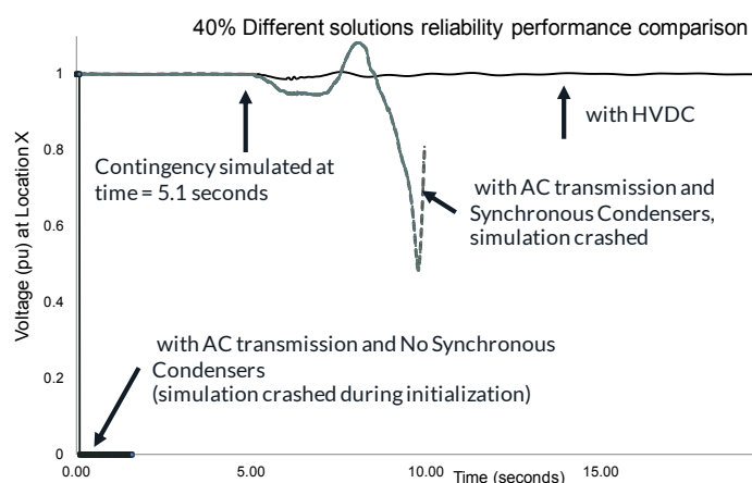
Figure OR-DS-7: Power delivery from low short circuit areas may need HVDC transmission technologies
