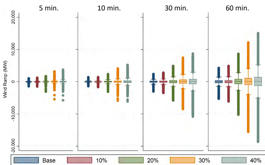
Figure EAD-4: Wind ramp for various renewable penetration milestones
