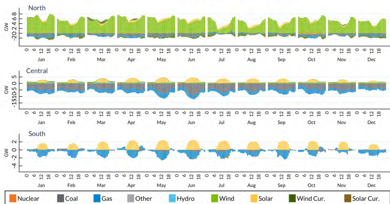
Figure EA-18: Monthly diurnal average of fuel mix, incremental change from the 30% milestone to the 40% milestone
