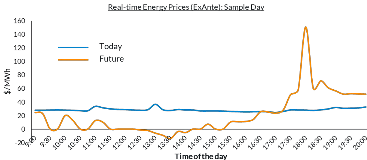
Figure EAM-4: Comparison of ex-ante real-time energy prices, today vs future (sample day)
