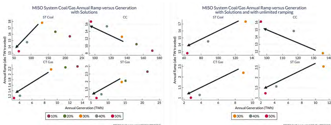
Figure EA-12: Thermal unit ramping in RIIA milestones, assuming unlimited ramping capabilities for all thermal units
