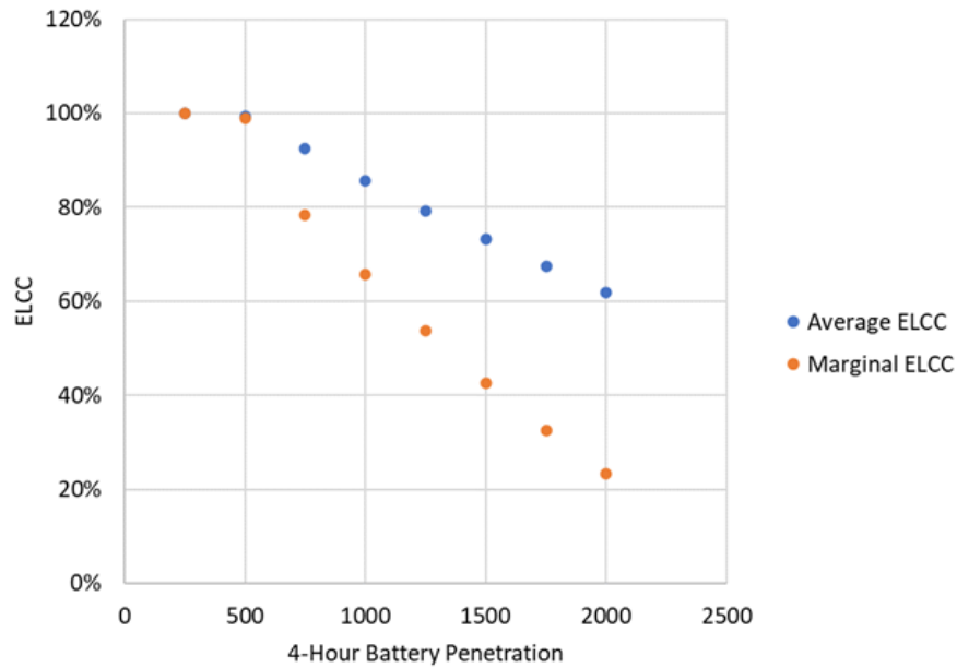
Figure 4. Battery ELCC by Cumulative Capacity Deployed
