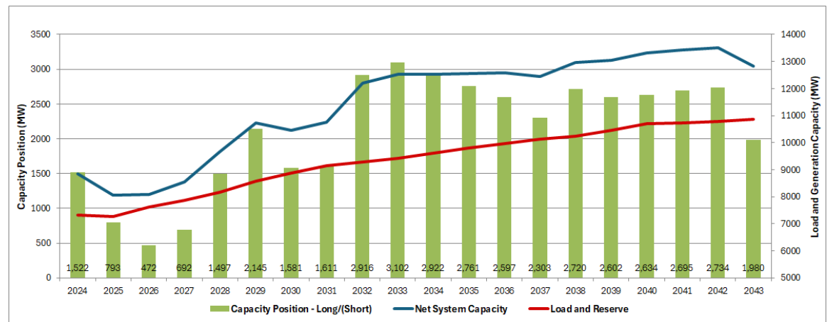
3 4 Figure 8. Summer Capacity Position – Load Case 4 – All Planned Resources 5 – Normal Weather
