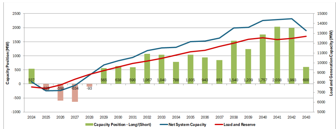
10 Figure 2. Winter Capacity Position – Load Case 5 11
