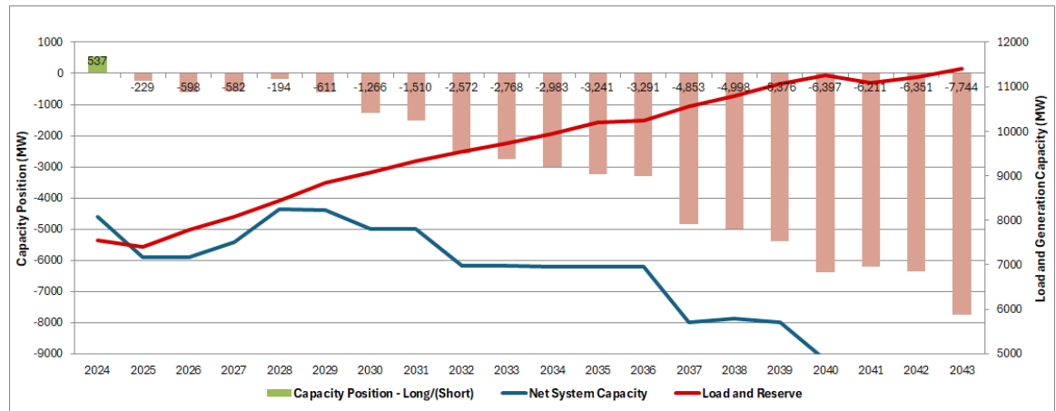
Figure 5. Winter Capacity Position – Load Case 4 – Existing and Approved Resources – Normal Weather
