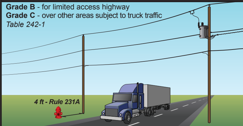
Vertical Clearance at Largest Vertical Sag Table 232-1
